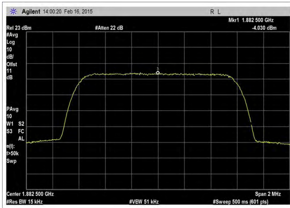
7.10_OBW_UL_1850-1915MHz_CDMA_Output
