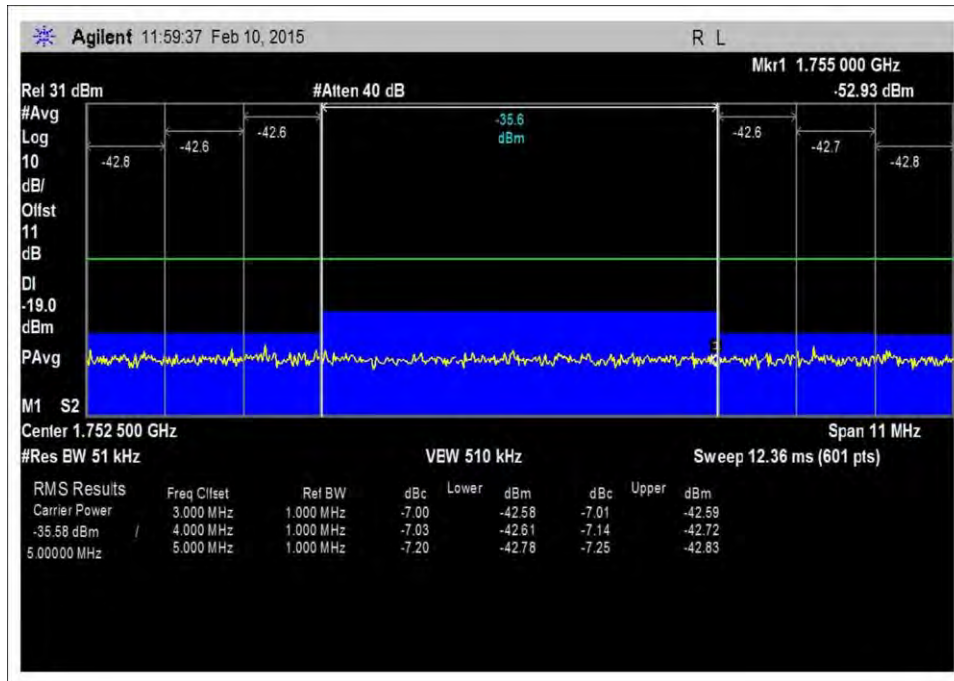
7.5_OBE_UL_1710-1755MHz_LTE_H_+10dBm
