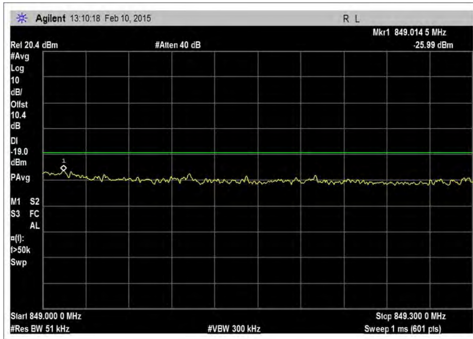
7.5_OBE_UL_824-849MHz_LTE_H_-26dBm
