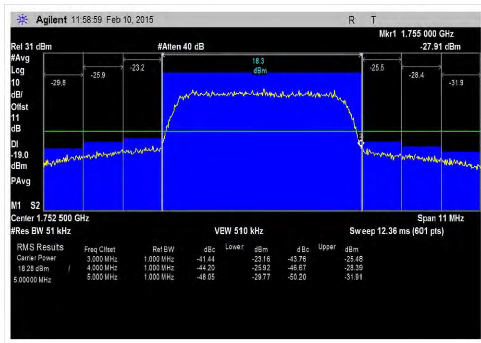
7.5_OBE_UL_1710-1755MHz_LTE_H_-20dBm
