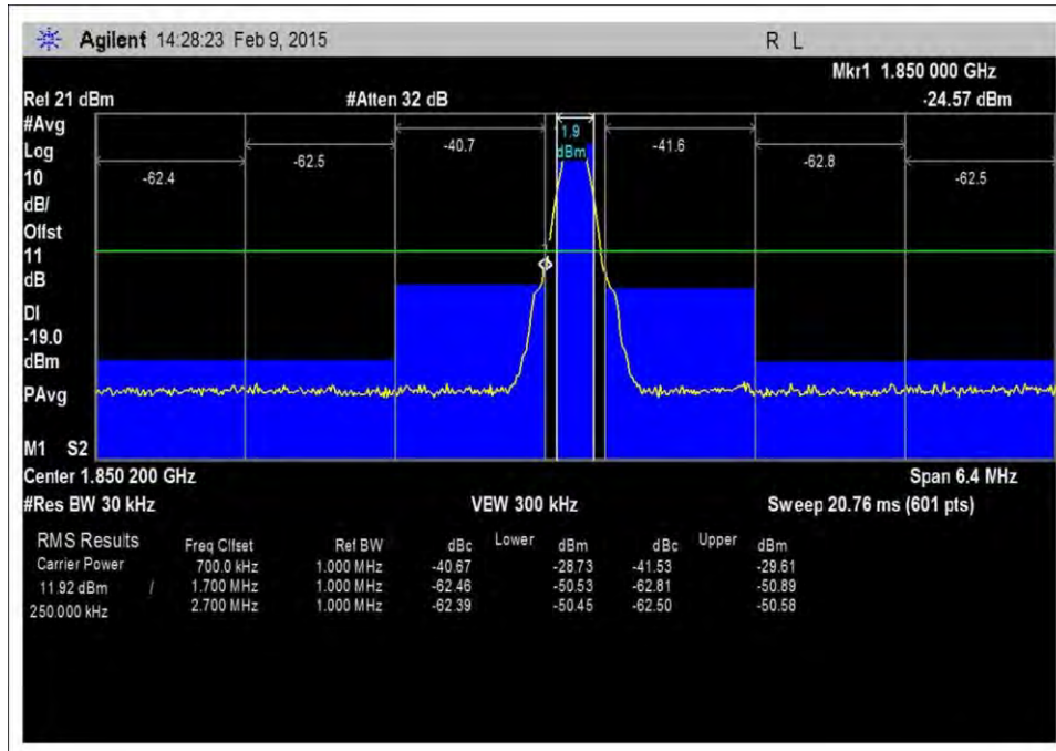
7.5_OBE_UL_1850-1915MHz_GSM_L_-27dBm
