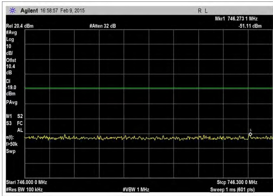
7.5_OBE_DL_728-746MHz_GSM_H_-20dBm
