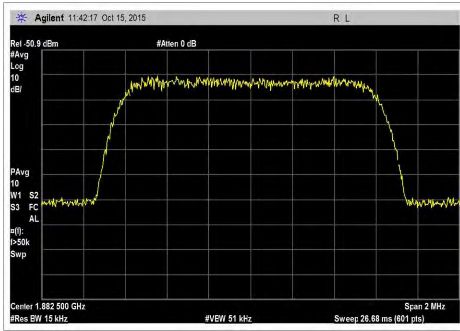
7.10_OBW_UL_1850-1915MHz_CDMA
