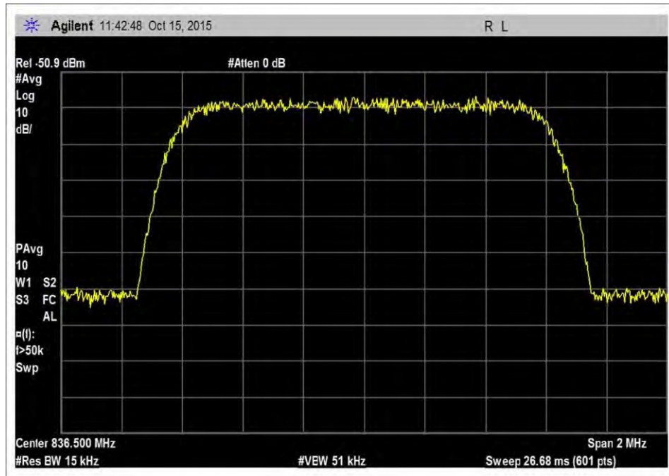
7.10_OBW_UL_824-849MHz_CDMA
