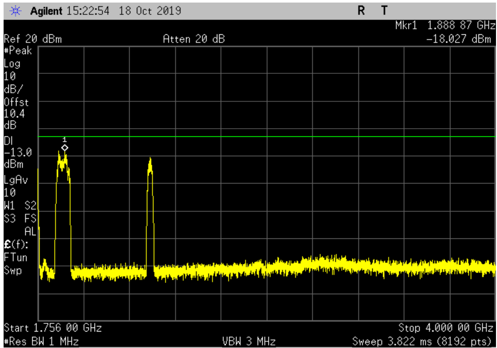
UL_1710-1755_GSM_1756-4000MHz_HC
