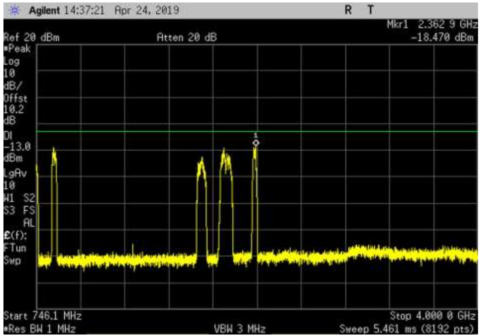
DL_728-746_GSM_746.1-4000MHz_LC
