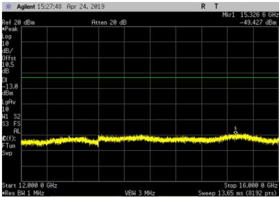
DL_2110-2155_AWGN_12000-16000MHz_MC
