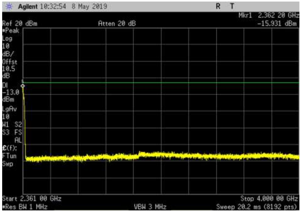
DL_2350-2360_AWGN_2361- 4000MHz_MC
