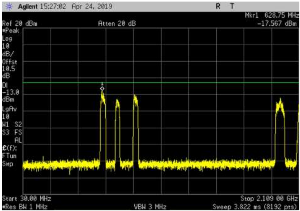
DL_2110-2155_AWGN_30- 2109MHz_MC
