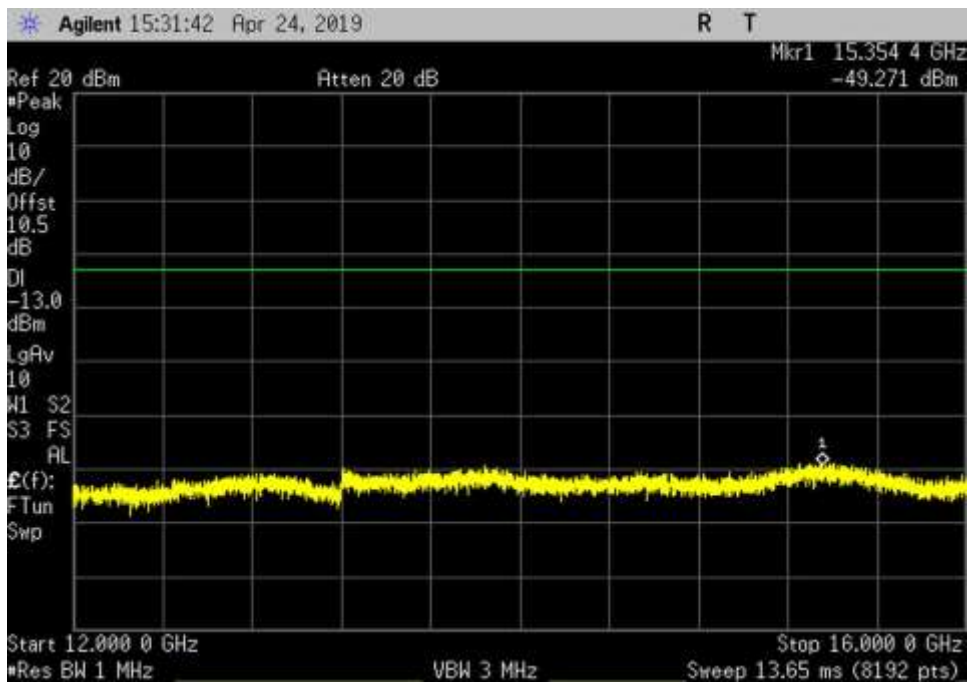
DL_1930-1995_AWGN_12000-16000MHz_LC
