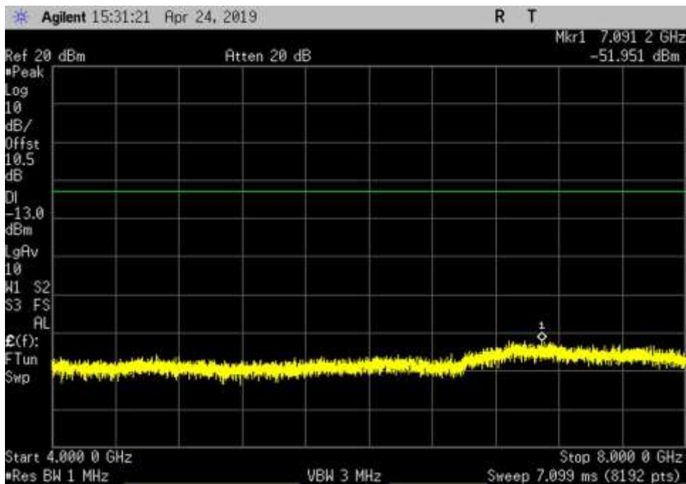
DL_1930-1995_AWGN_4000-8000MHz_LC
