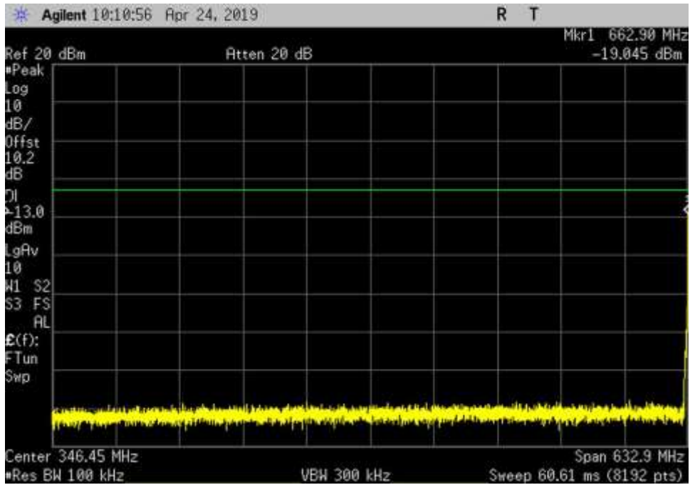
UL_663-698_GSM_30- 662.9MHz_LC
