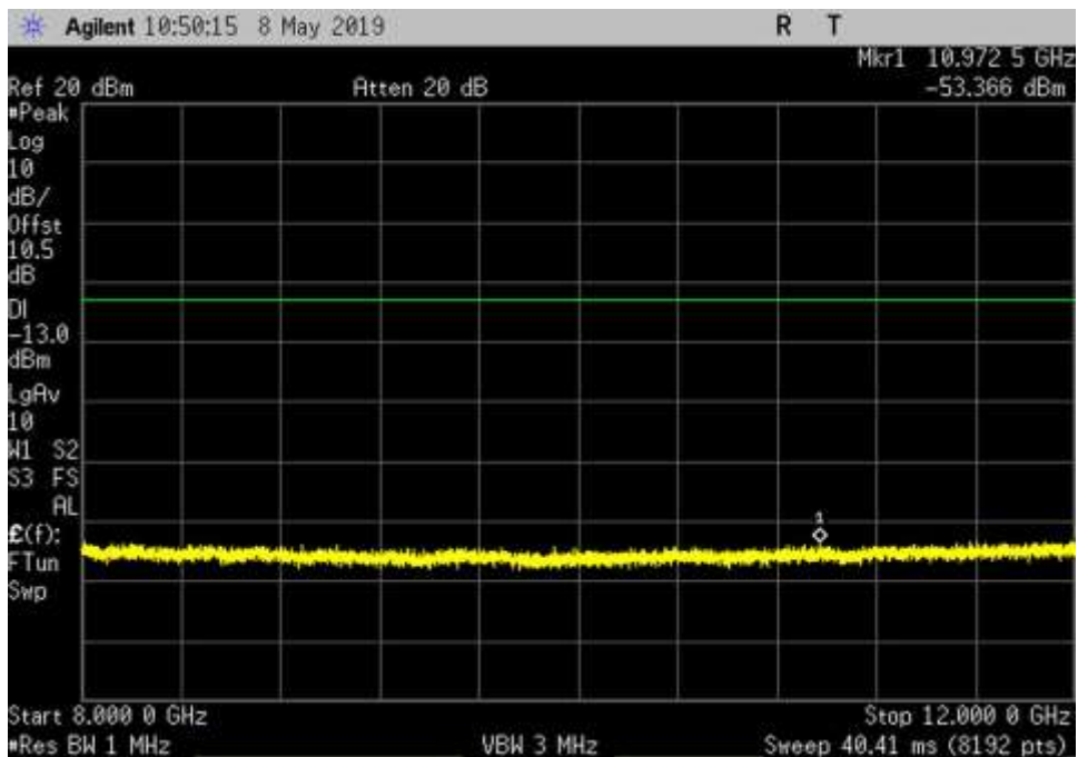
UL_2305-2315_GSM_8000-12000MHz_LC
