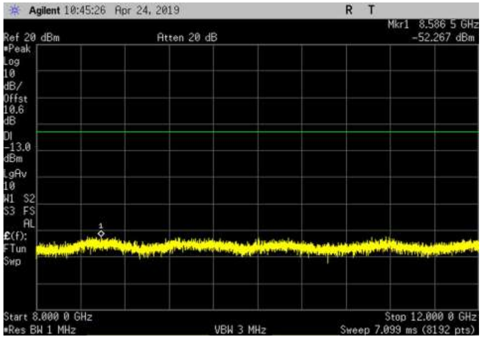
UL_1850-1915_GSM_8000-12000MHz_MC
