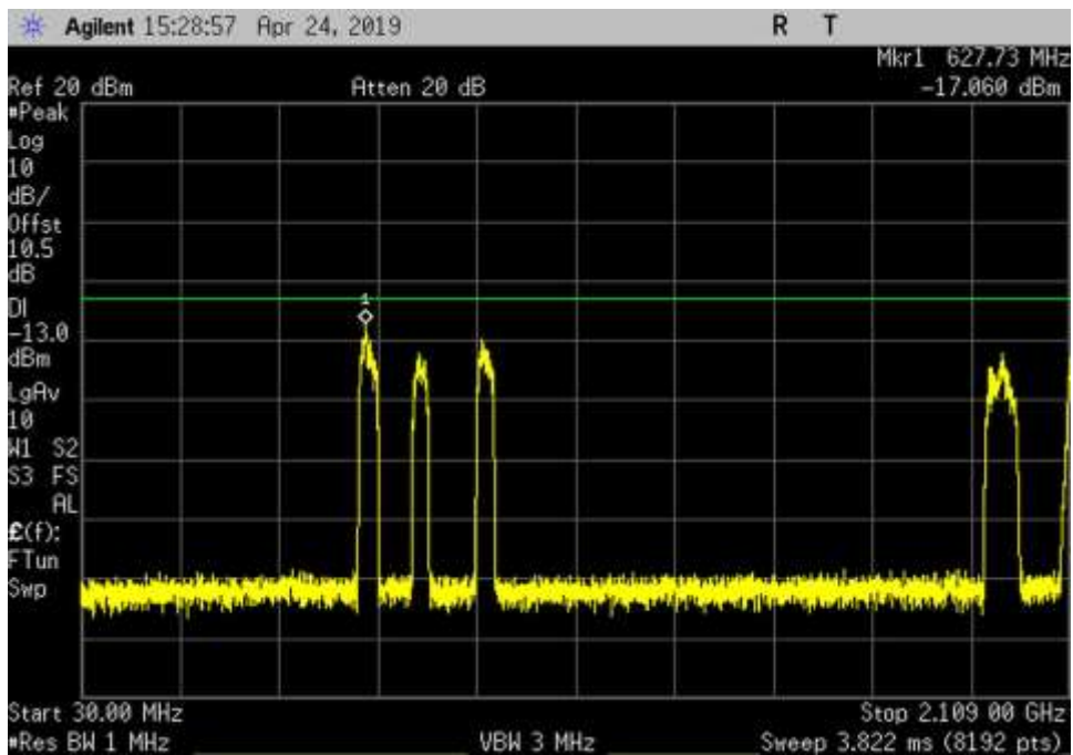
DL_2110-2155_AWGN_30- 2109MHz_HC
