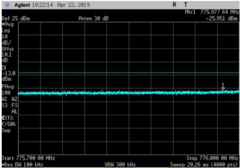
UL_776-787_AWGN_775.7-776MHz_Sn-L
