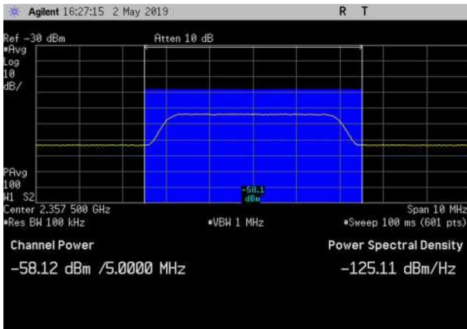
DL_2350-2360_AWGN_ 2357.5MHz_Input
