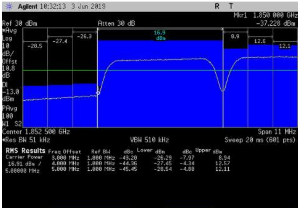
UL_1850-1915_AWGN_1847-1850MHz_Cm-L+3dB
