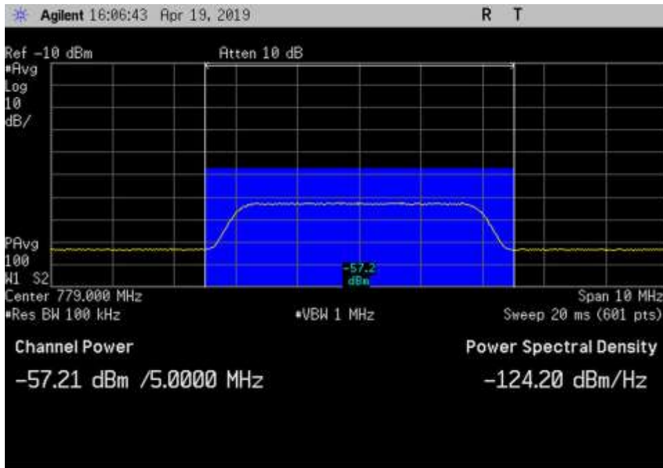
UL_776-787_AWGN_779MHz_Input
