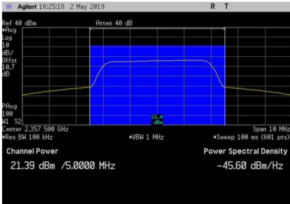
DL_2350-2360_AWGN_ 2357.5MHz_3dB
