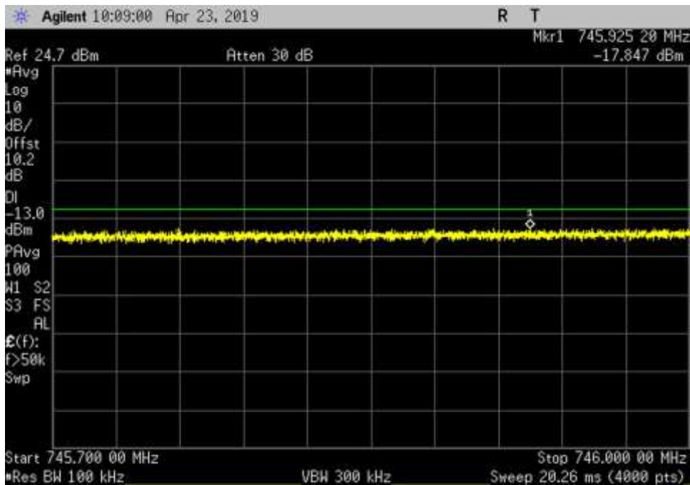
DL_746-757_AWGN_745.7-746MHz_Sn-L+3dB
