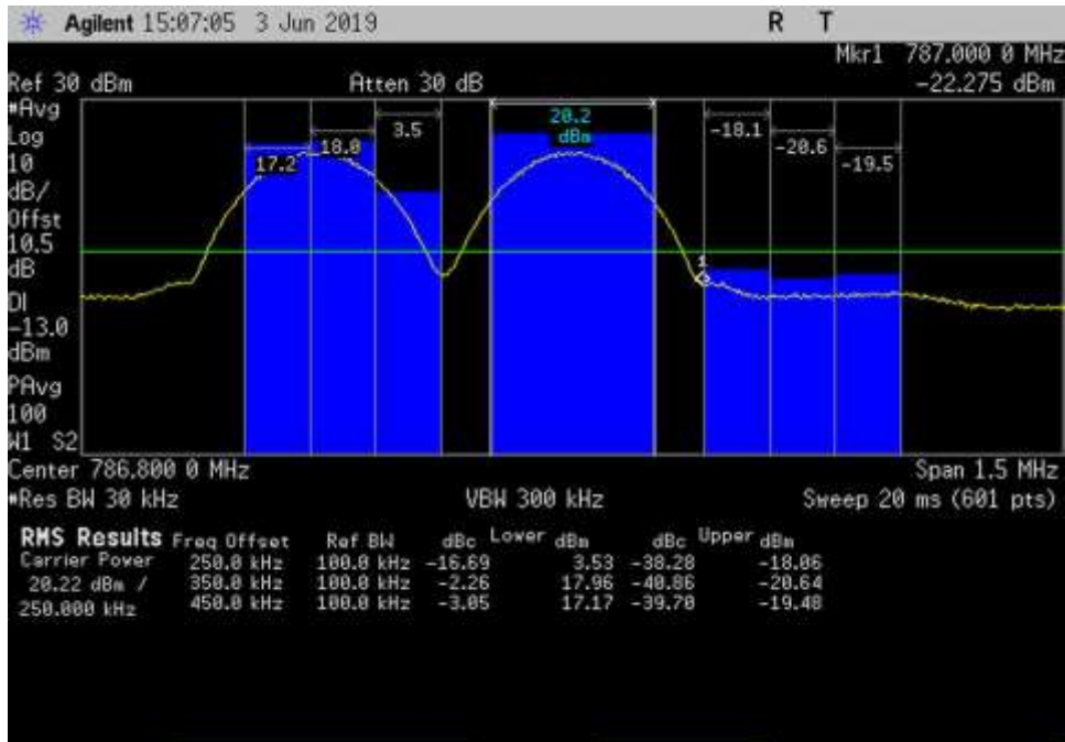
UL_776-787_GSM_787-787.3MHz_Cm-H+3dB
