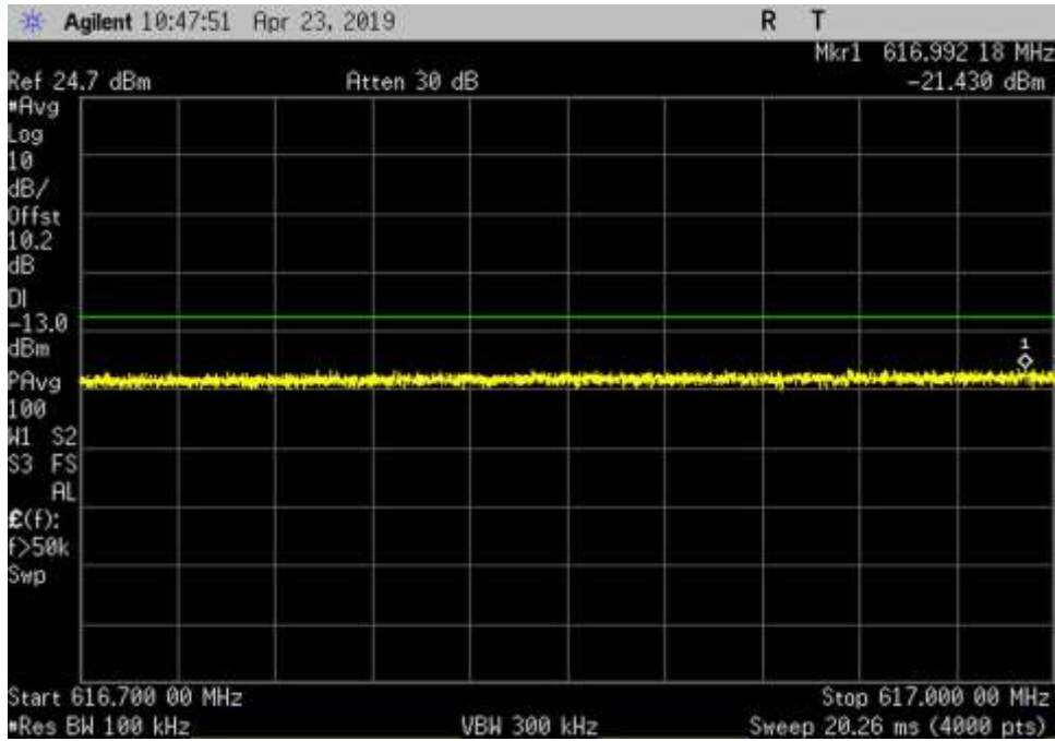
DL_617-652_AWGN_616.7-617MHz_Cm-L
