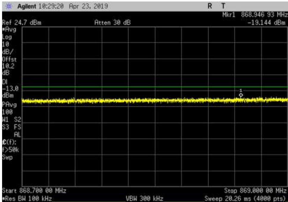
DL_869-894_AWGN_ 868.7- 869MHz_Sn-L+3dB
