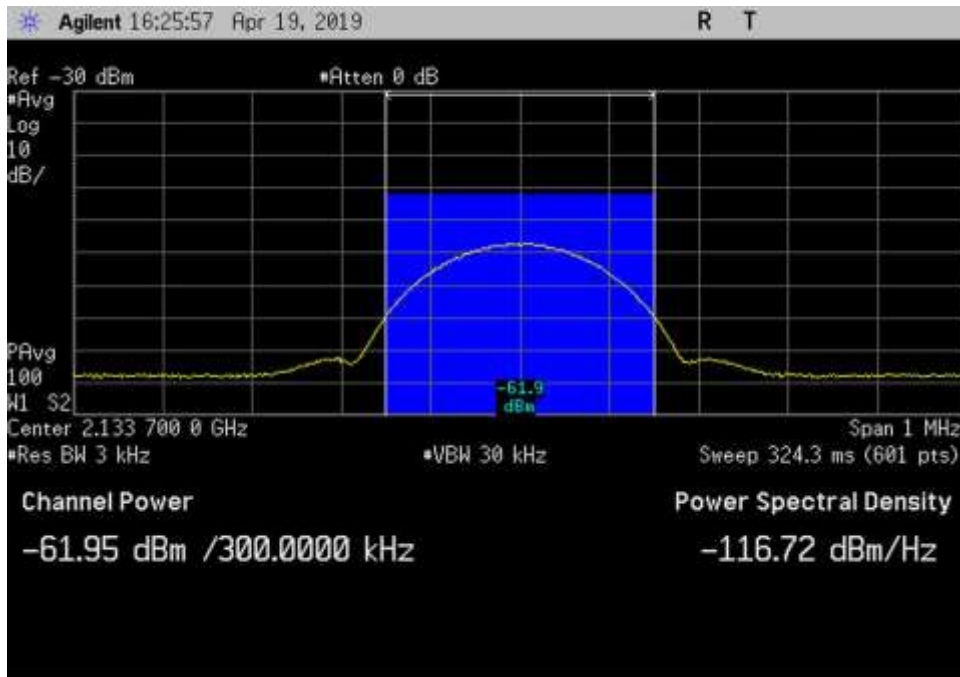
DL_2110-2155_GSM_2133.7MHz_Input
