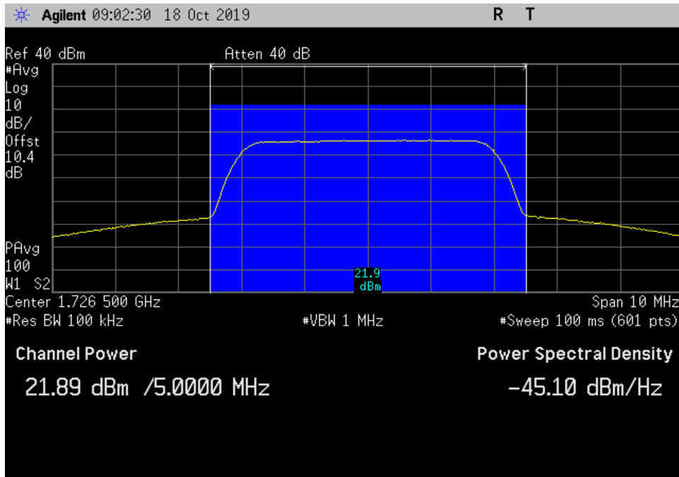
UL_1710-1755_AWGN_1726.5MHz_3dB
