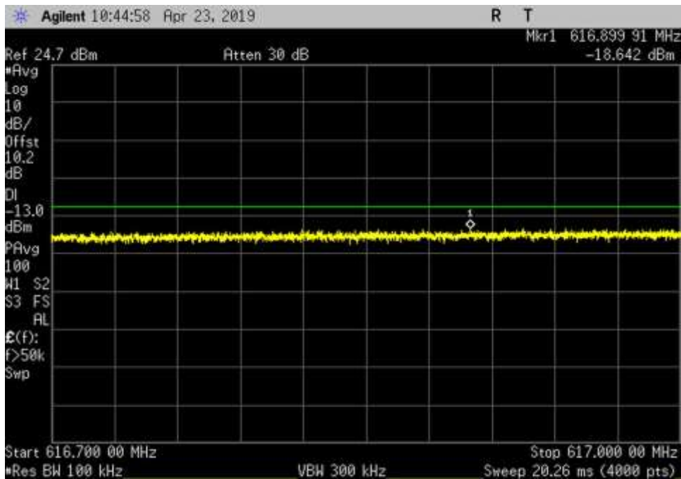
DL_617-652_AWGN_616.7-617MHz_Sn-L+3dB
