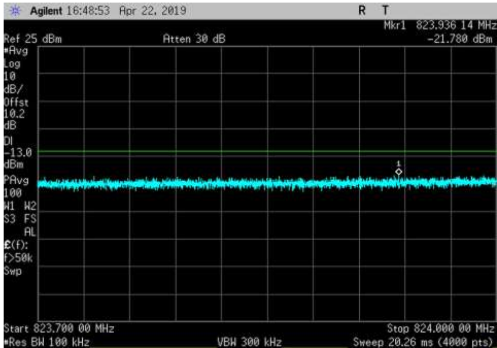
UL_824-849_AWGN_ 823.7- 824MHz_Sn-L+3dB
