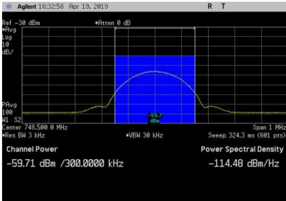
DL_746-757_GSM_748.5MHz_Input
