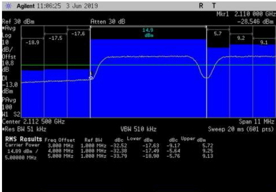
DL_2110-2155_AWGN_2107-2110MHz_Cm-L+3dB
