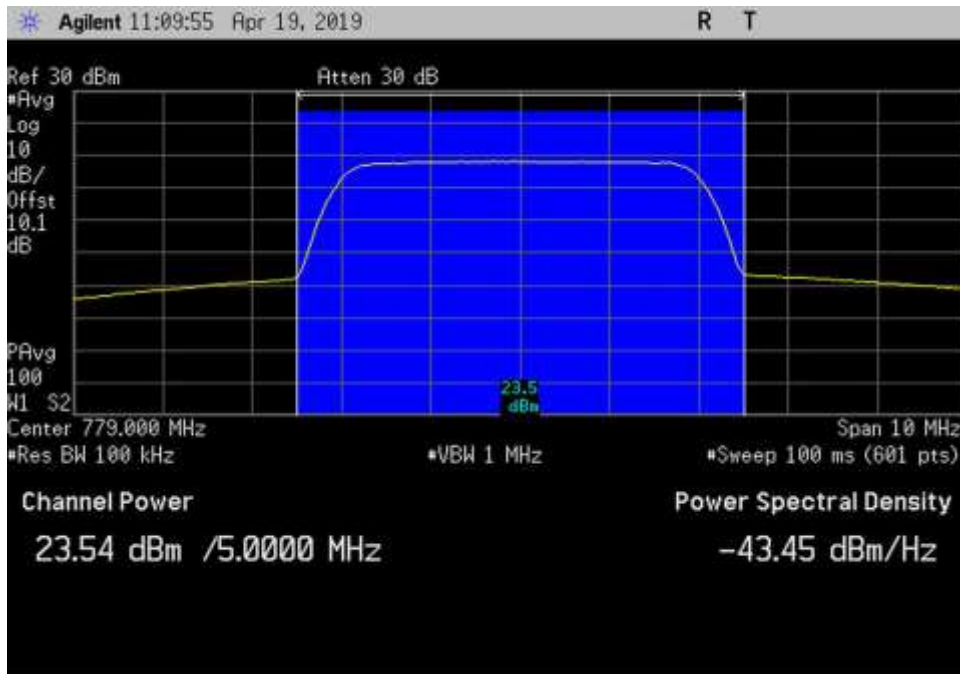
UL_776-787_AWGN_779MHz_3dB
