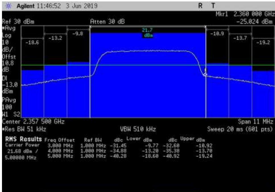
DL_2350-2360_AWGN_2360-2363MHz_Sn-H+3dB
