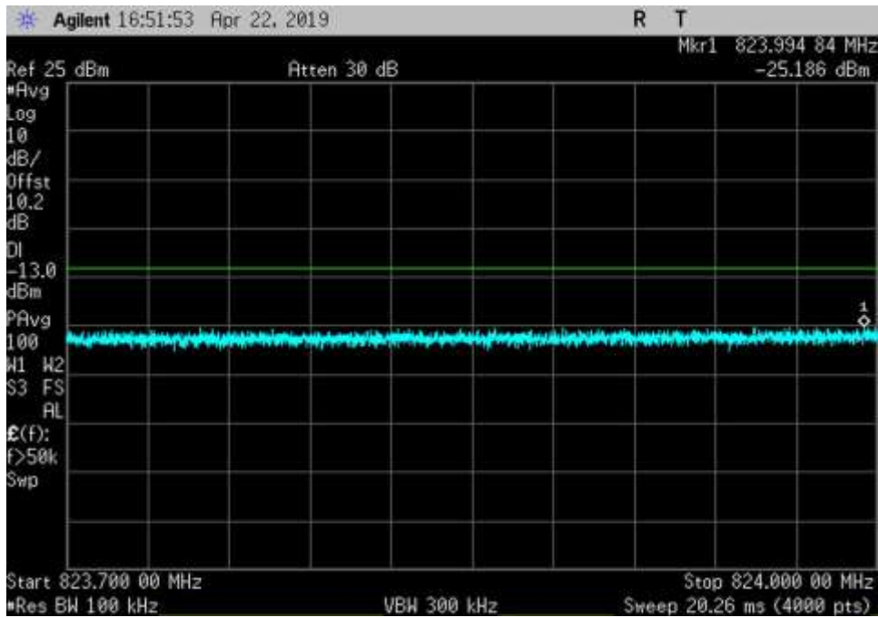
UL_824-849_AWGN_823.7-824MHz_Cm-L
