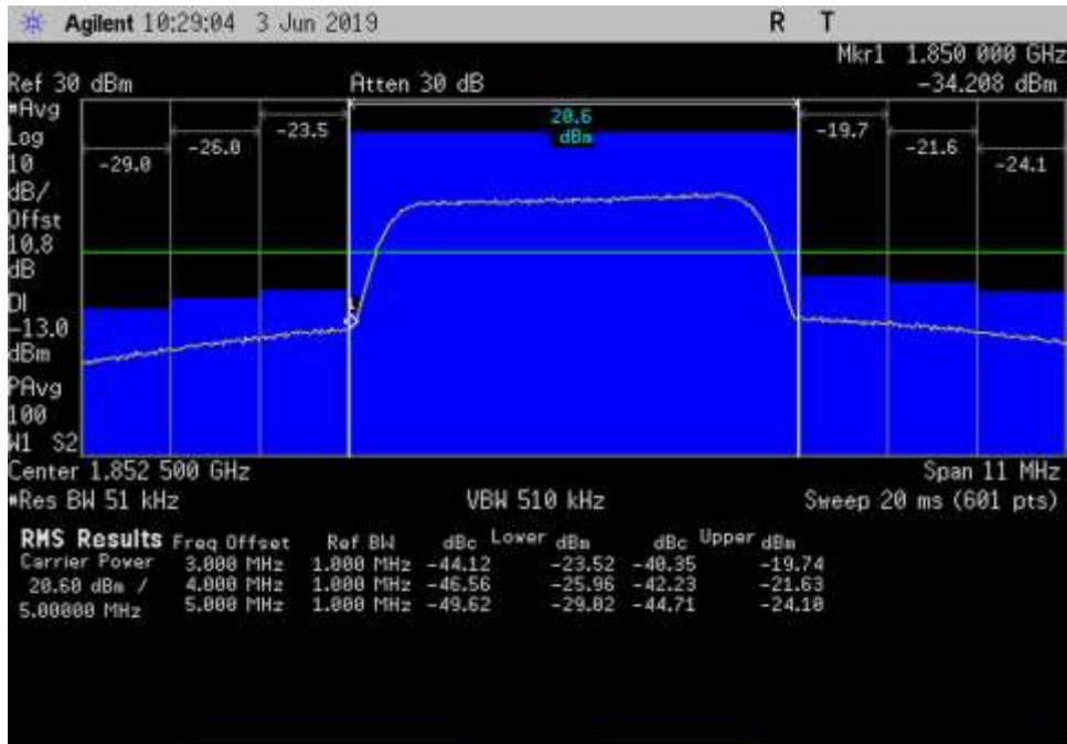
UL_1850-1915_AWGN_1847-1850MHz_Sn-L+3dB
