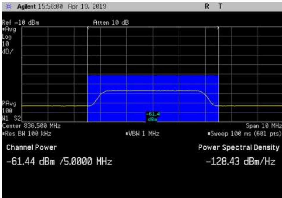
UL_824-849_AWGN_836.5MHz_Input
