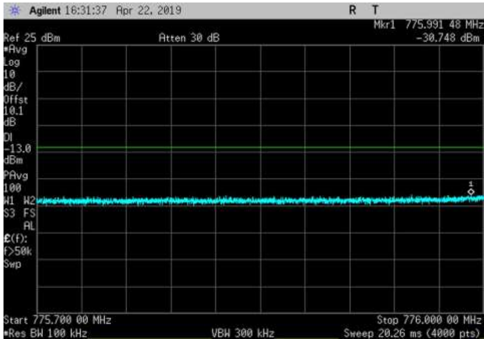
UL_776-787_AWGN_775.7-776MHz_Cm-L+3dB
