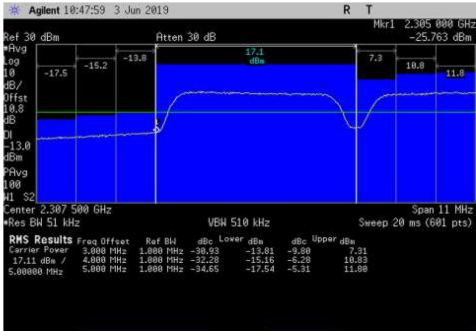
UL_2305-2315_AWGN_2302-2305MHz_Cm-L+3dB
