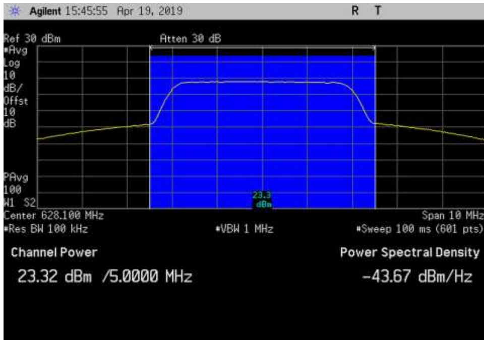
DL_617-652_AWGN_628.1MHz
