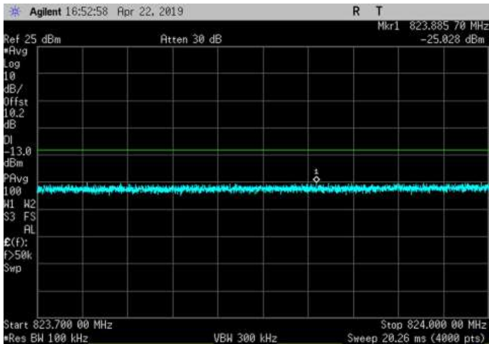
UL_824-849_AWGN_823.7-824MHz_Cm-L+3dB
