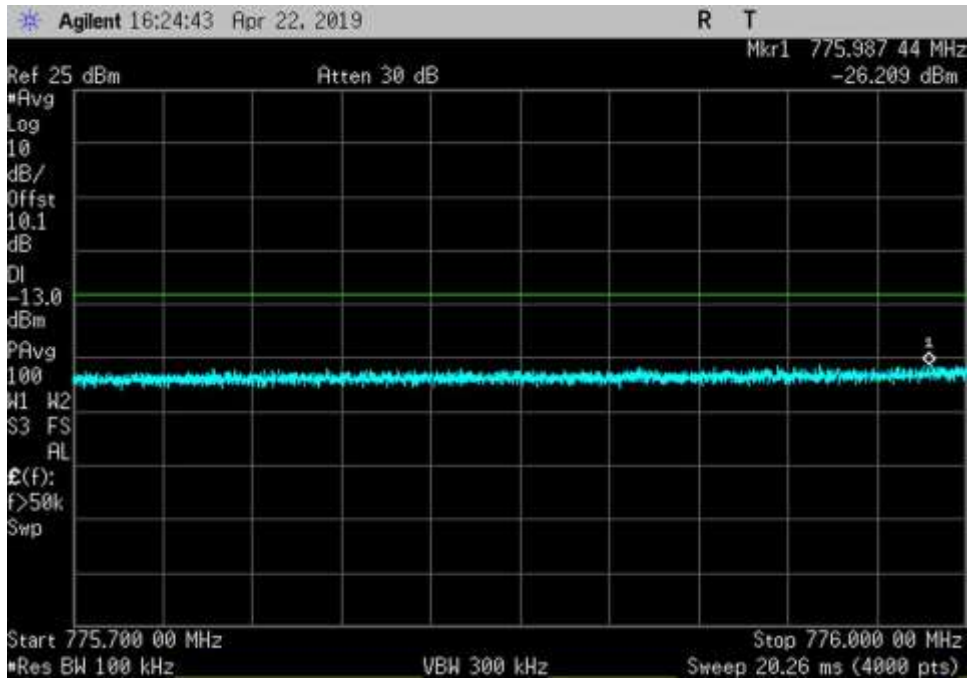
UL_776-787_AWGN_775.7-776MHz_Sn-L+3dB
