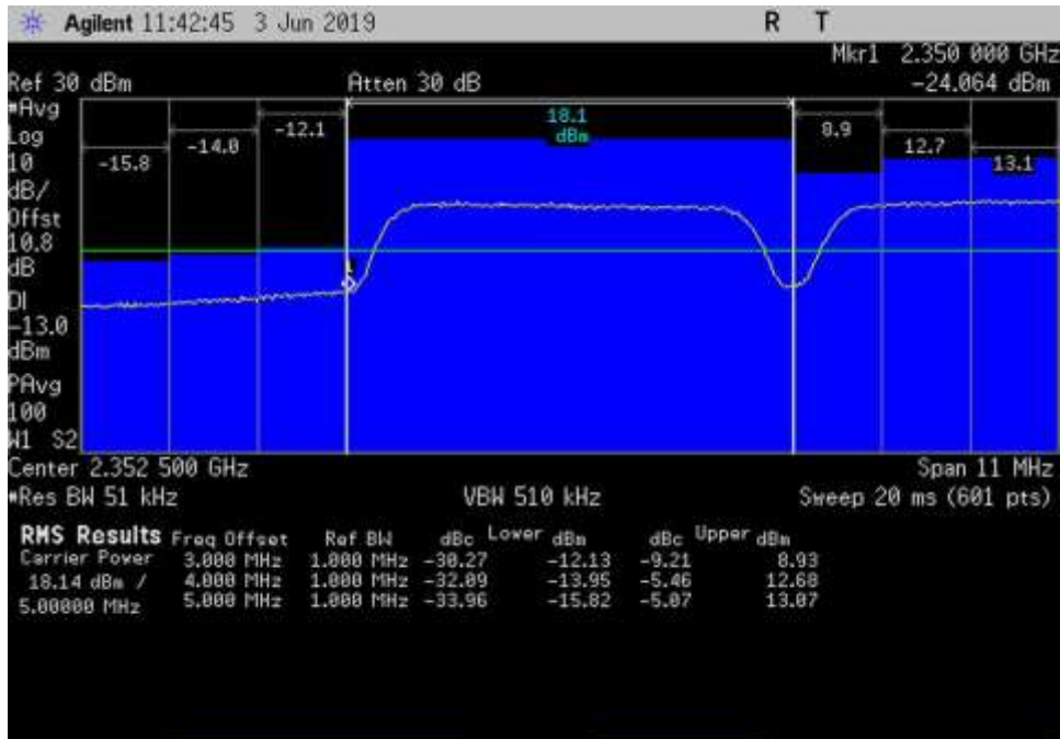
DL_2350-2360_AWGN_2347-2350MHz_Cm-L+3dB
