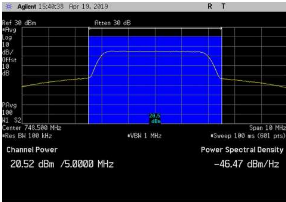
DL_746-757_AWGN_748.5MHz_3dB
