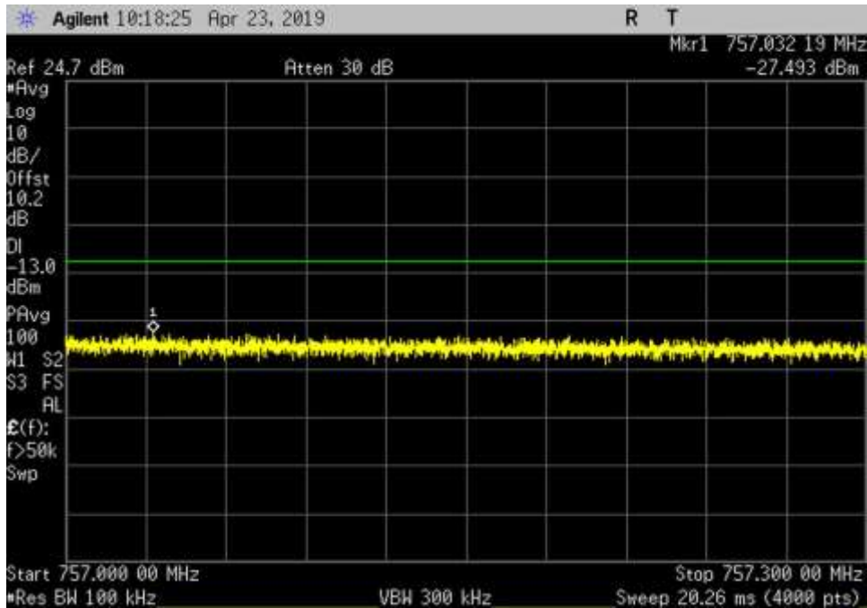
DL_746-757_AWGN_757- 757.3MHz_Sn-H+3dB
