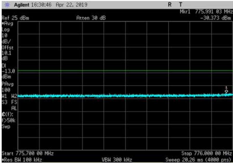
UL_776-787_AWGN_775.7-776MHz_Cm-L
