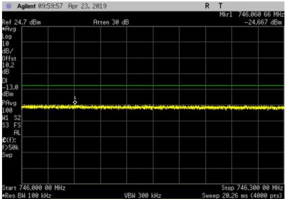
DL_728-746_AWGN_746-746.3MHz_Cm-H+3dB
