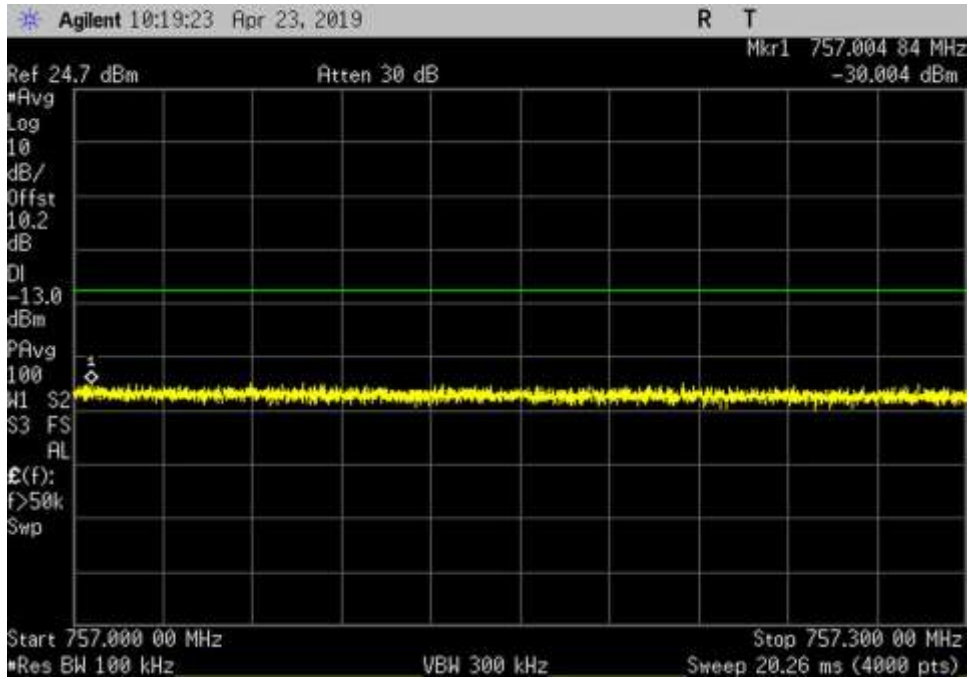
DL_746-757_AWGN_ 757- 757.3MHz_Cm-H
