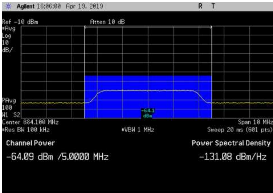
UL_663-698_AWGN_ 684.1MHz_Input
