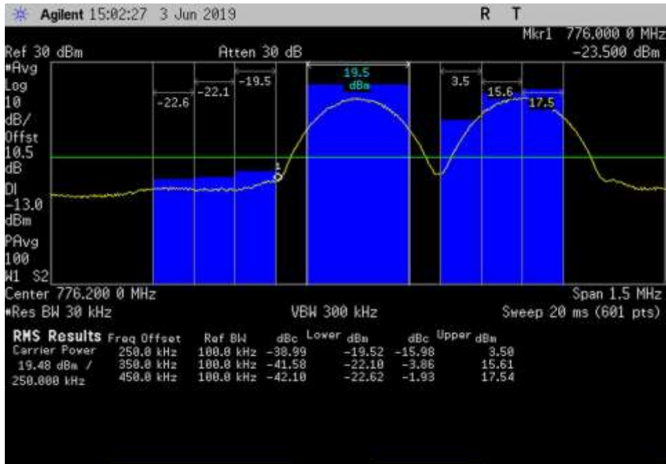
UL_776-787_GSM_775.7-776MHz_Cm-L+3dB
