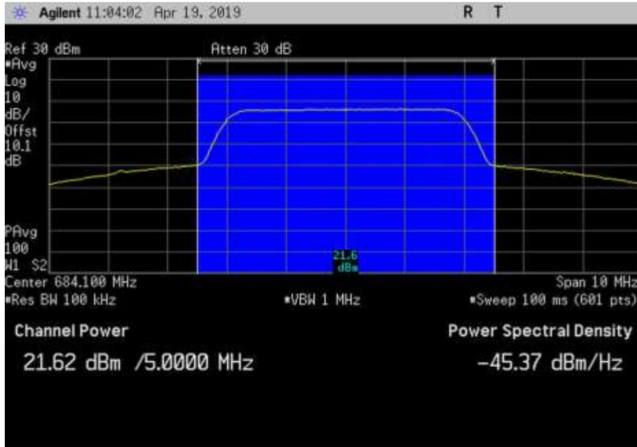
UL_663-698_AWGN_684.1MHz
