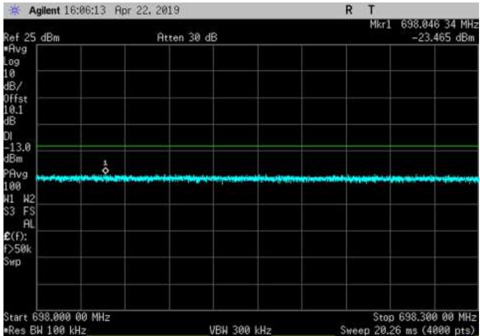
UL_663-698_AWGN_698-698.3MHz_Cm-H+3dB
