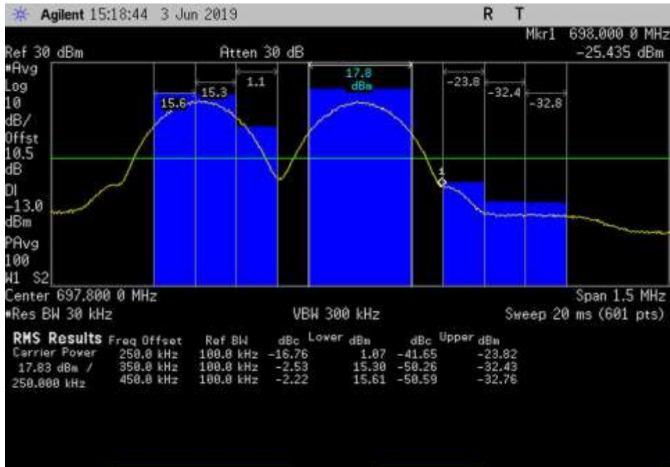
UL_663-698_GSM_698-698.3MHz_Cm-H+3dB
