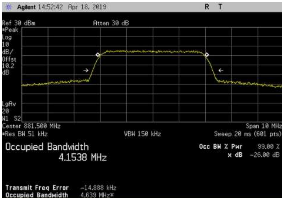
Out_DL_869-894_AWGN_881.5MHz
