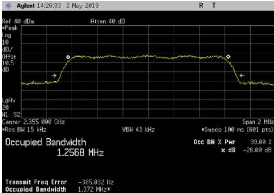
Out_DL_2350-2360_CDMA_2355MHz
