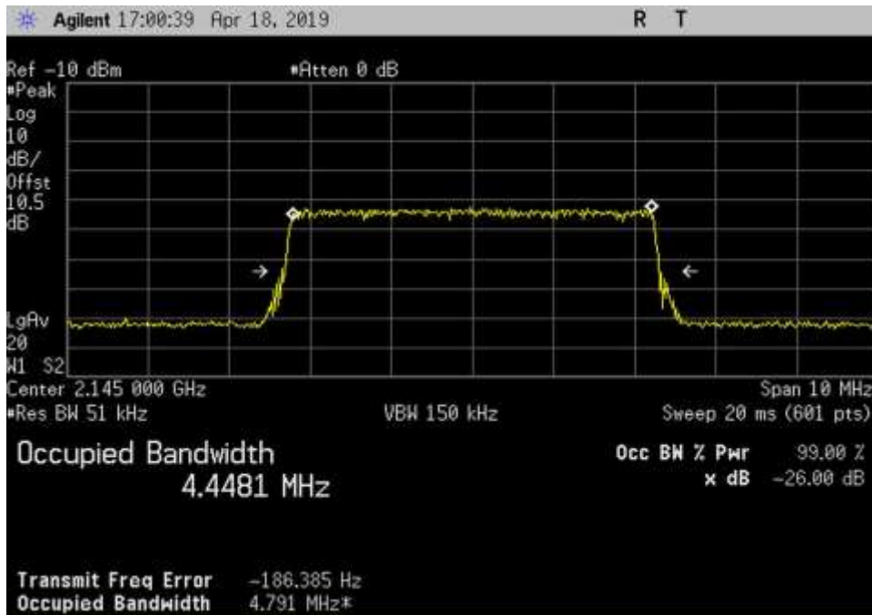
In_DL_2110-2155_LTE_2145MHz
