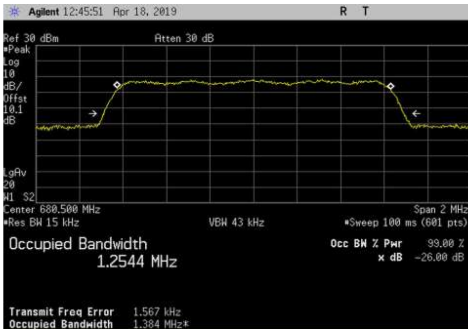
Out_UL_663-698_CDMA_680.5MHz_3dB
