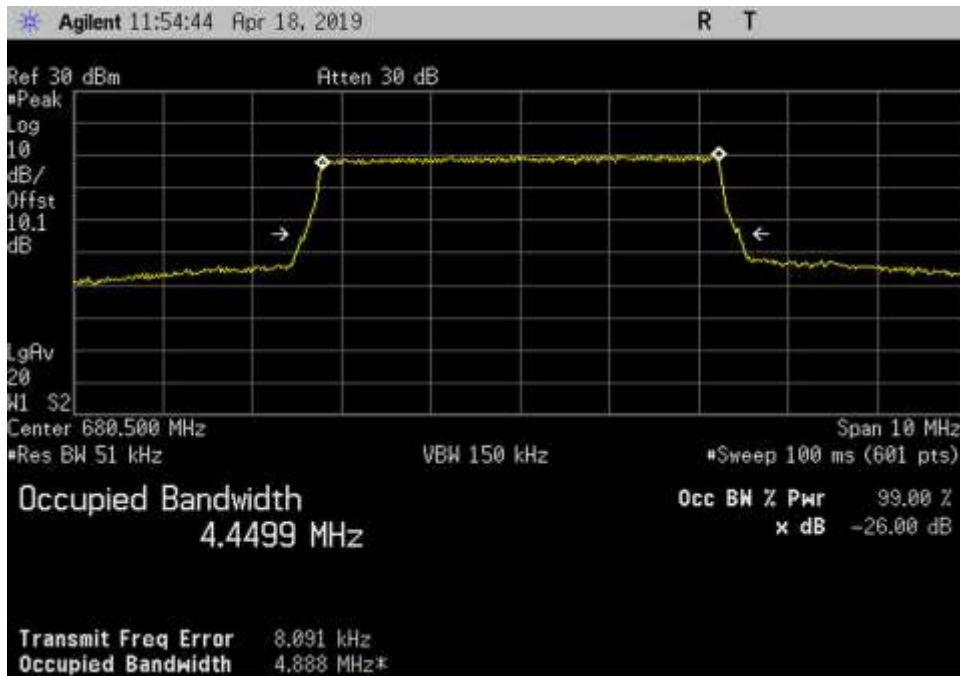
Out_UL_663-698_LTE_680.5MHz_3dB
