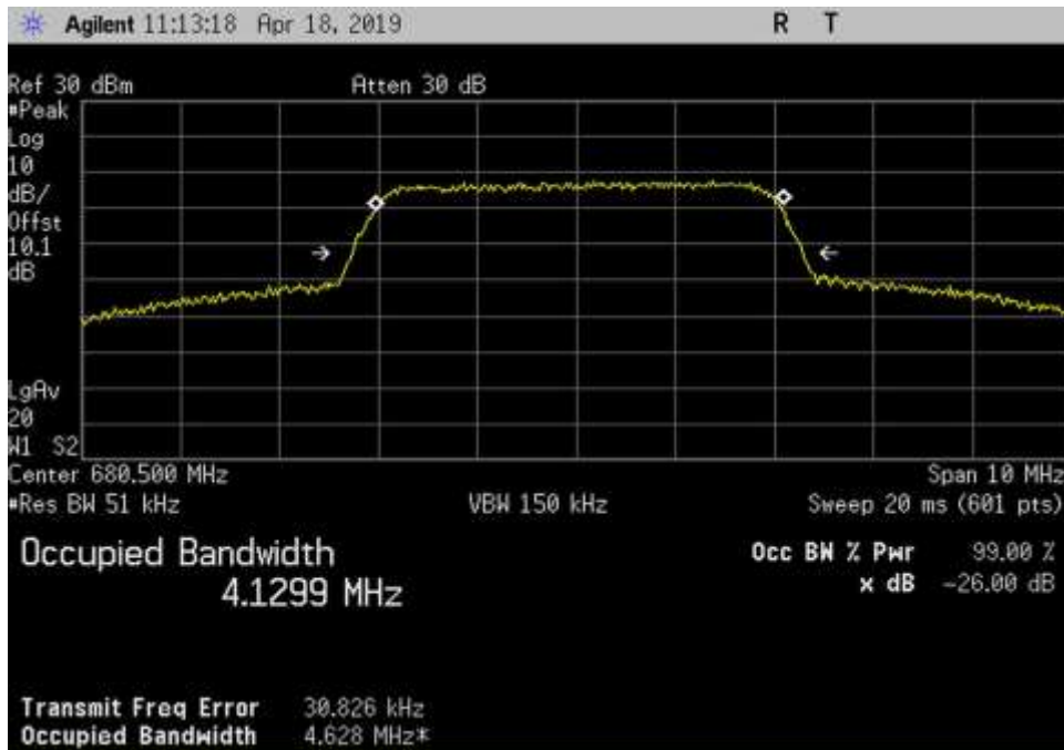
Out_UL_663-698_AWGN_680.5MHz_3dB
