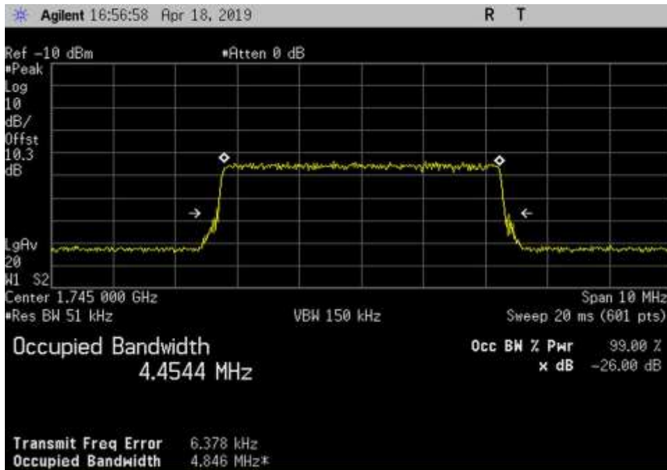
In_UL_1710-1755_LTE_1745MHz
