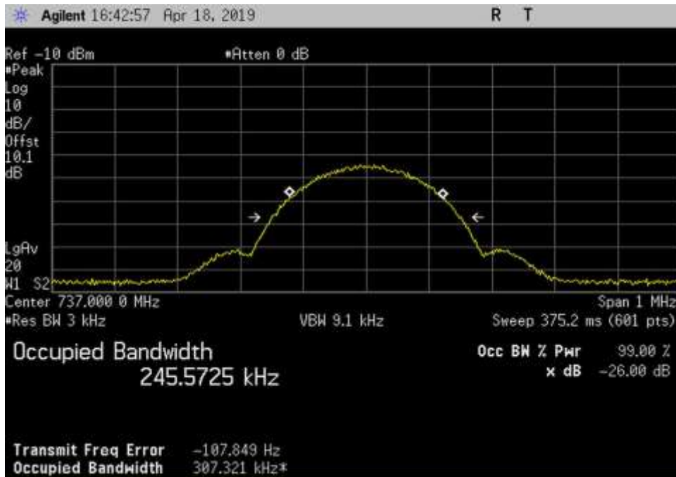
In_DL_728-746_GSM_737MHz
