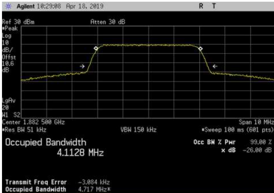
Out_UL_1850-1915_AWGN_1882.5MHz_3dB
