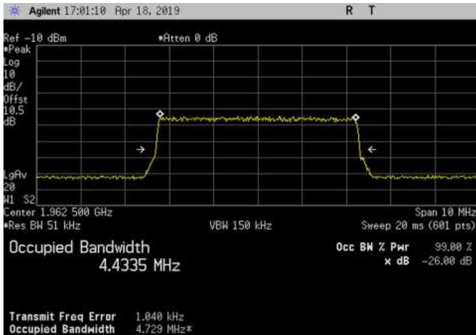
In_DL_1930-1995_LTE_1962.5MHz
