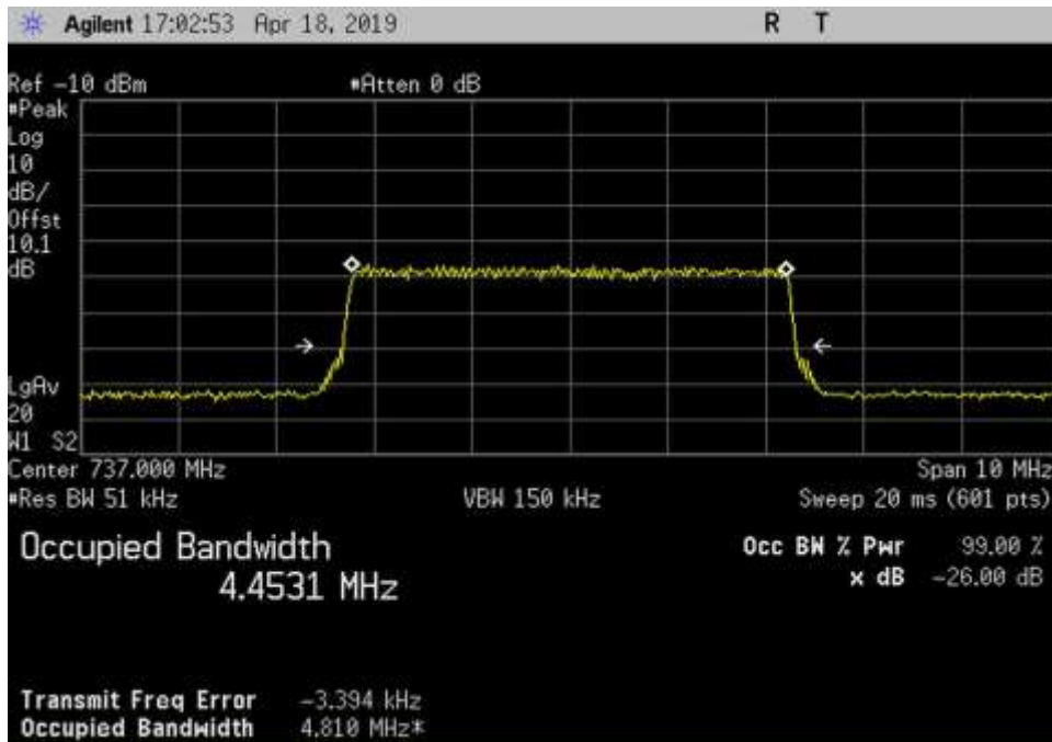
In_DL_728-746_LTE_737MHz
