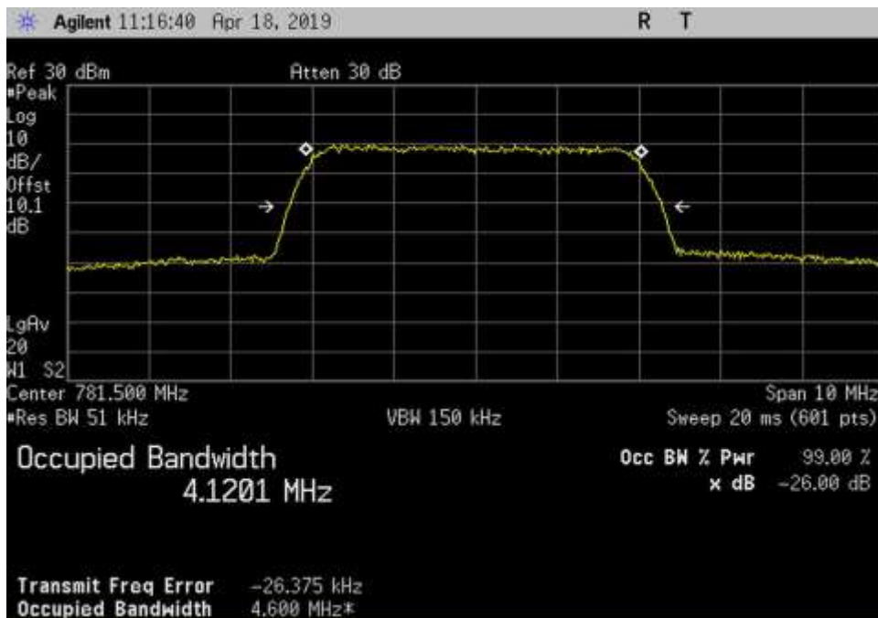
Out_UL_776-787_AWGN_781.5MHz
