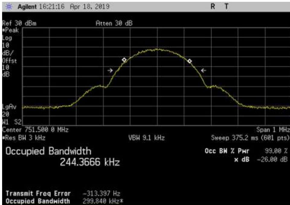
Out_DL_746-757_GSM_751.5MHz_3dB
