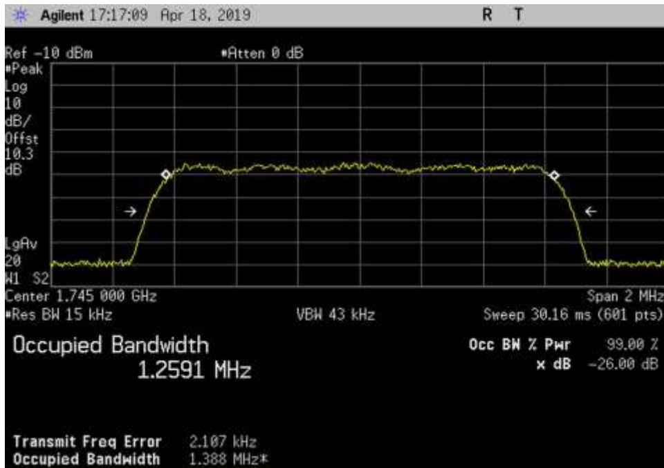
In_UL_1710-1755_CDMA_1745MHz
