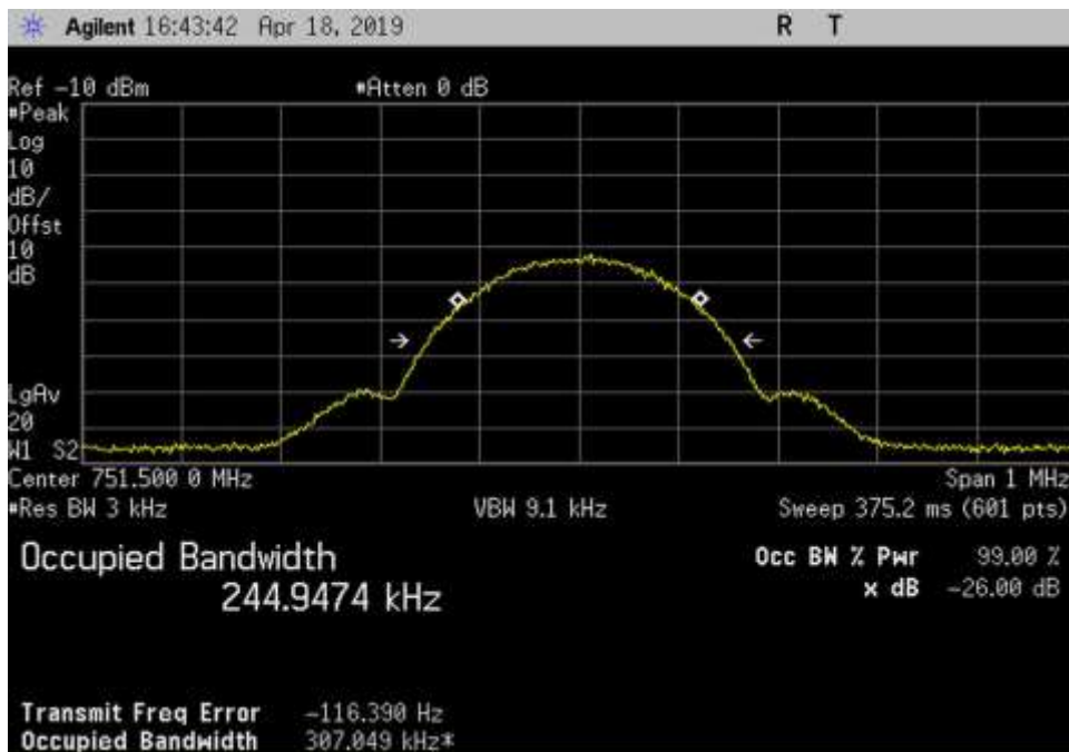
In_DL_746-757_GSM_751.5MHz
