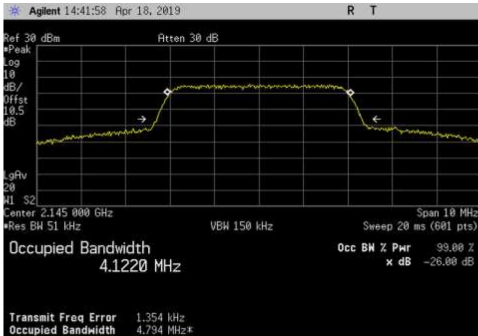
Out_DL_2110-2155_AWGN_2145MHz
