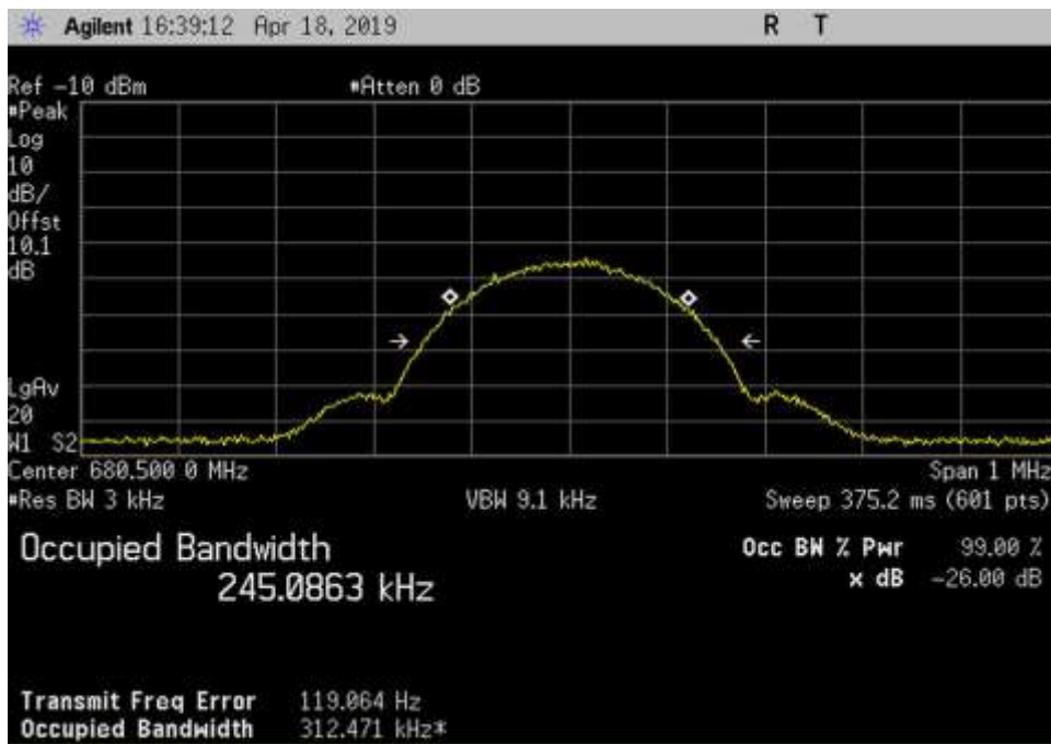
In_UL_663-698_GSM_680.5MHz
