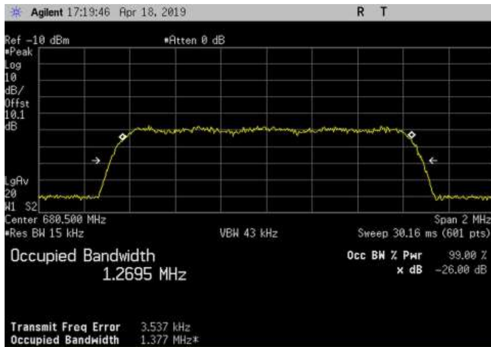
In_UL_663-698_CDMA_680.5MHz
