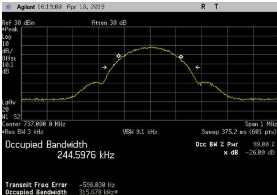
Out_DL_728-746_GSM_737MHz
