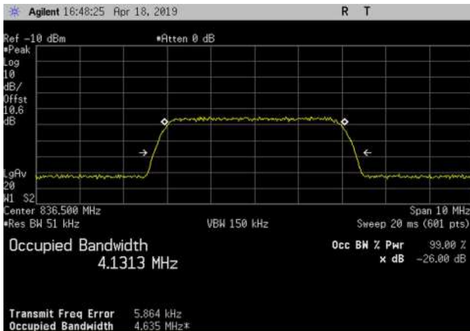
In_UL_824-849_AWGN_836.5MHz
