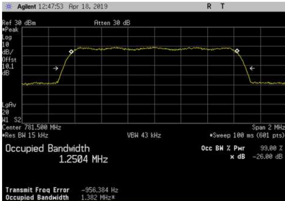
Out_UL_776-787_CDMA_781.5MHz_3dB
