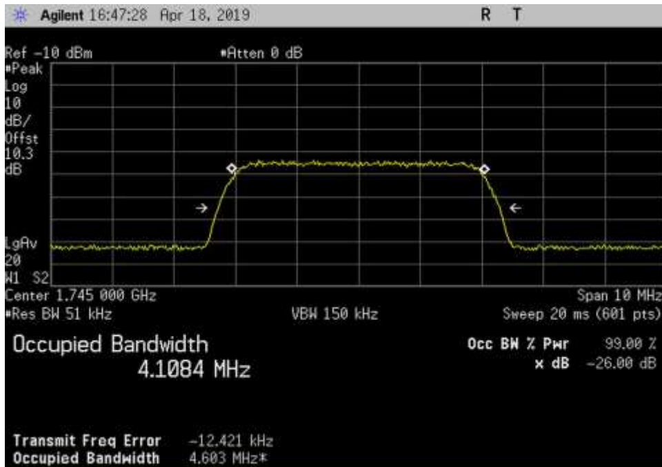
In_UL_1710-1755_AWGN_1745MHz
