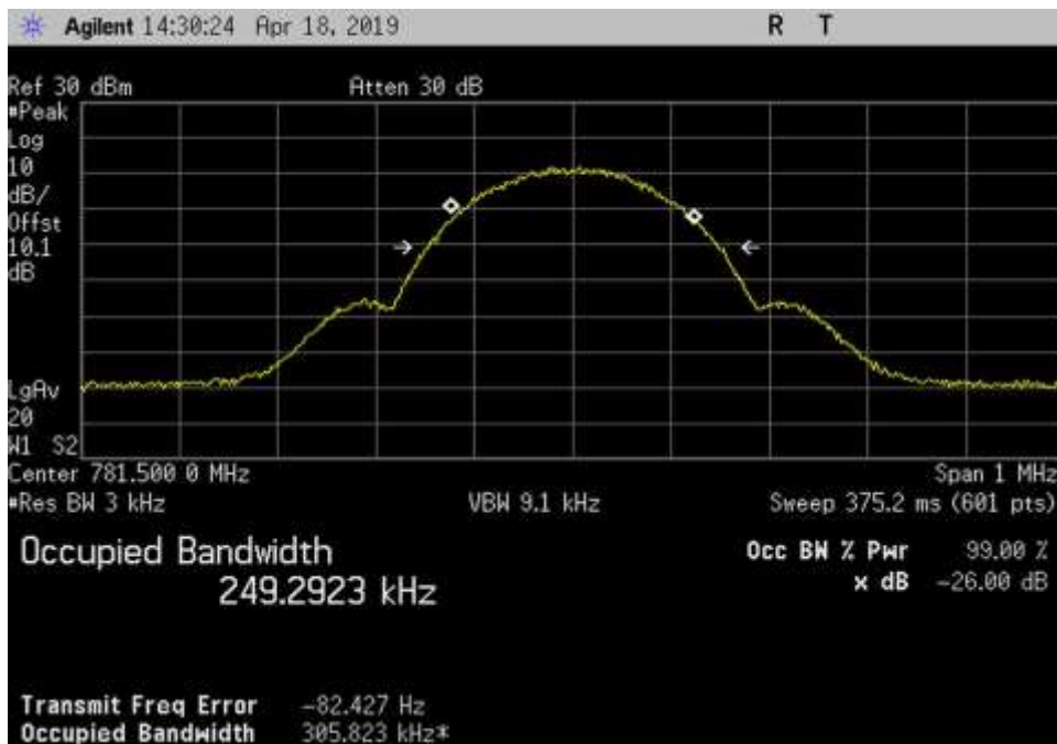
Out_UL_776-787_GSM_781.5MHz
