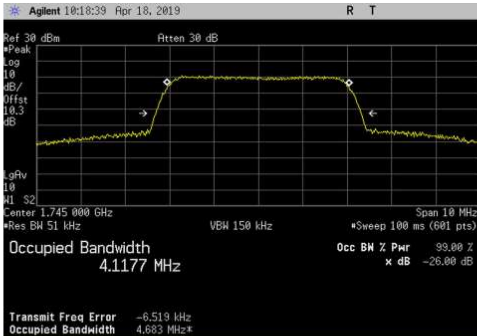
Out_UL_1710-1755_AWGN_1745MHz_3dB
