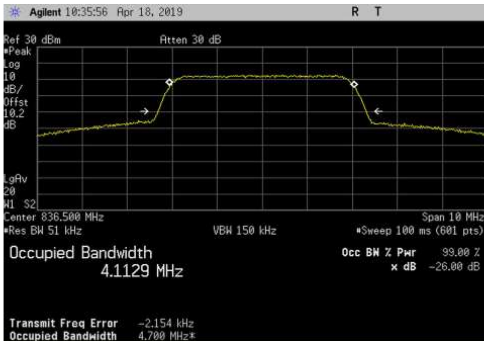
Out_UL_824-849_AWGN_836.5MHz
