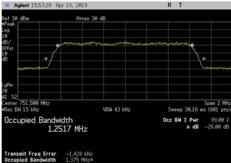
Out_DL_746-757_CDMA_751.5MHz
