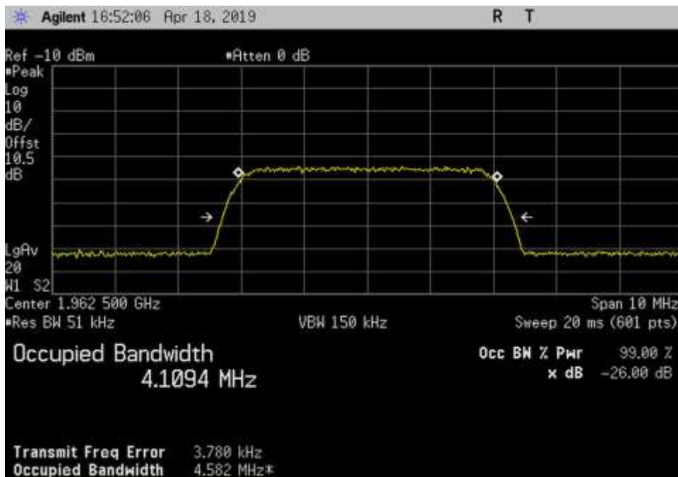
In_DL_1930-1995_AWGN_1962.5MHz
