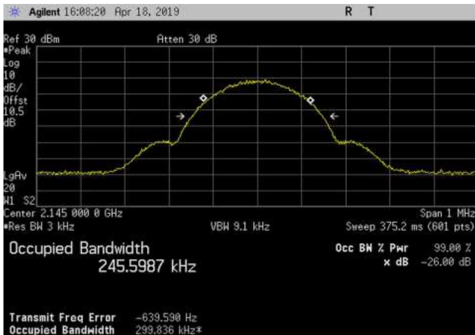
Out_DL_2110-2155_GSM_2145MHz
