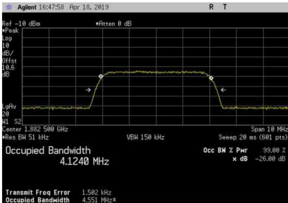
In_UL_1850-1915_AWGN_1882.5MHz
