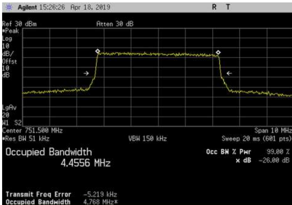
Out_DL_746-757_LTE_751.5MHz_3dB
