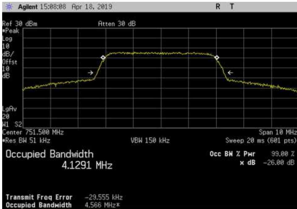
Out_DL_746-757_AWGN_751.5MHz_3dB
