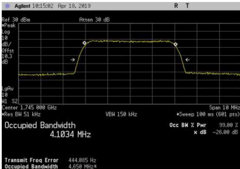
Out_UL_1710-1755_AWGN_1745MHz
