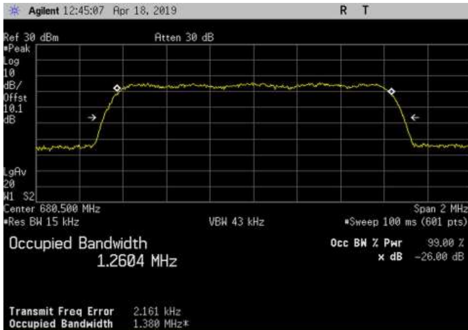
Out_UL_663-698_CDMA_680.5MHz
