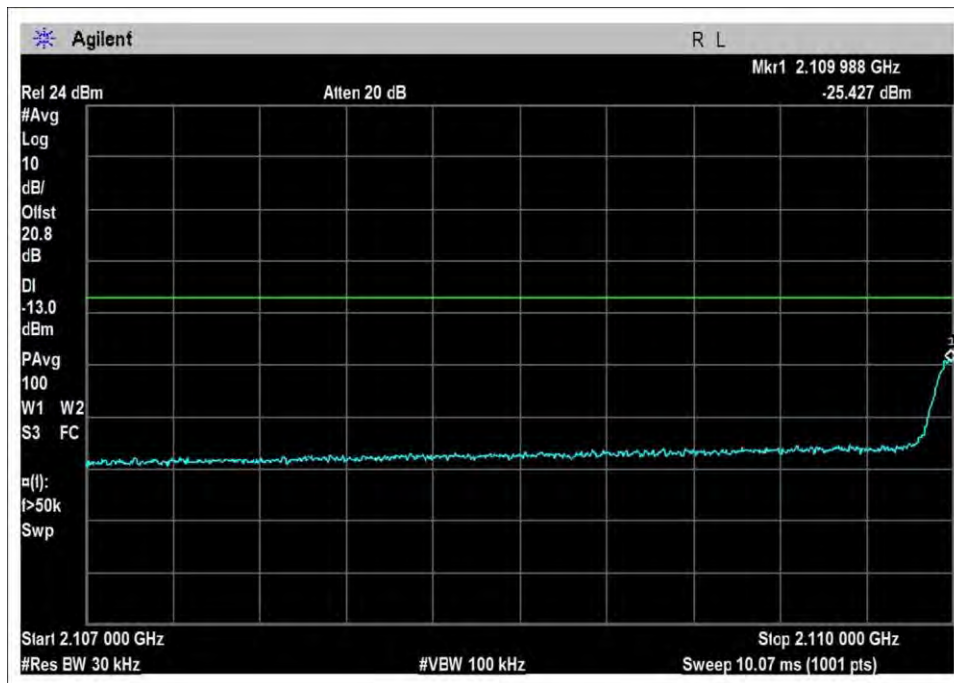
DL-2110-2155L-Sn-preAGC
