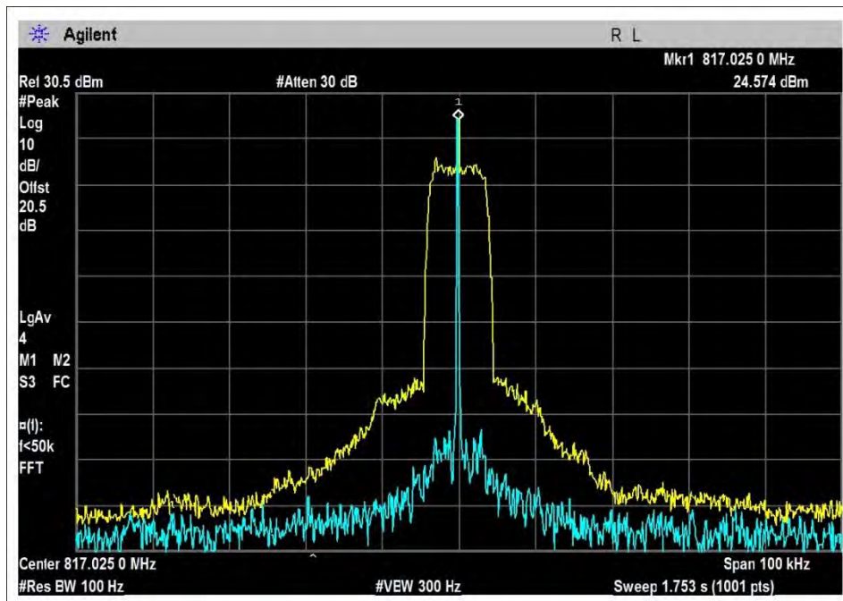
800M-F1W-UL-817-824L-Unmod
