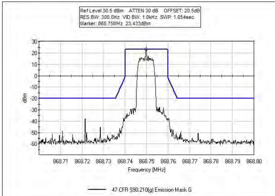
800M-F1W-DL-862-869H-MskG
