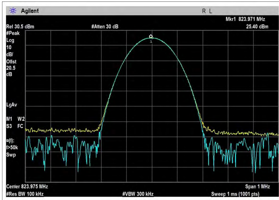
800M-F1W-UL-817-824H-Unmod
