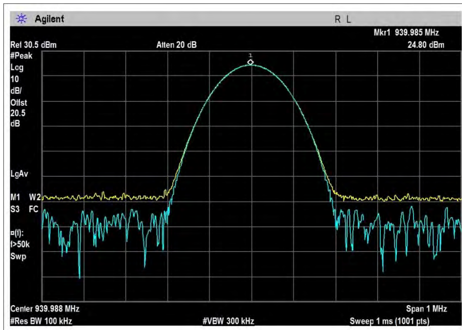
900M_FM_DL-940H-Unmod-35.1
