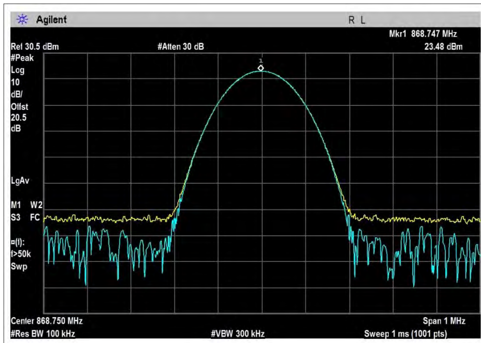
800M-F1W-DL-862-869H-Unmod
