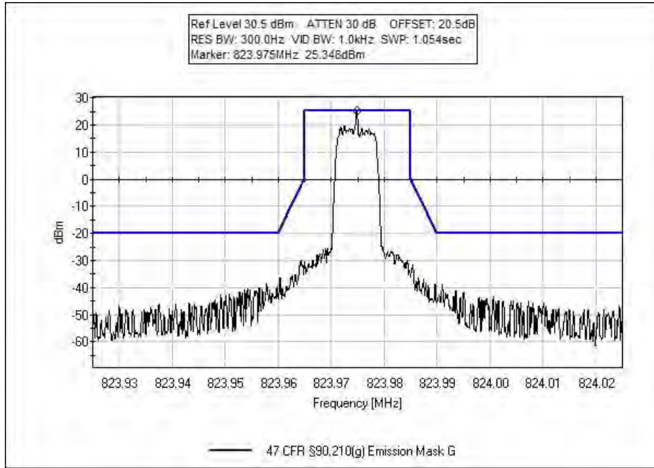
800M-F1W-UL-817-824H-MskG
