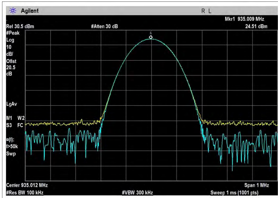
900M_FM_DL-935L-Unmod-31.5
