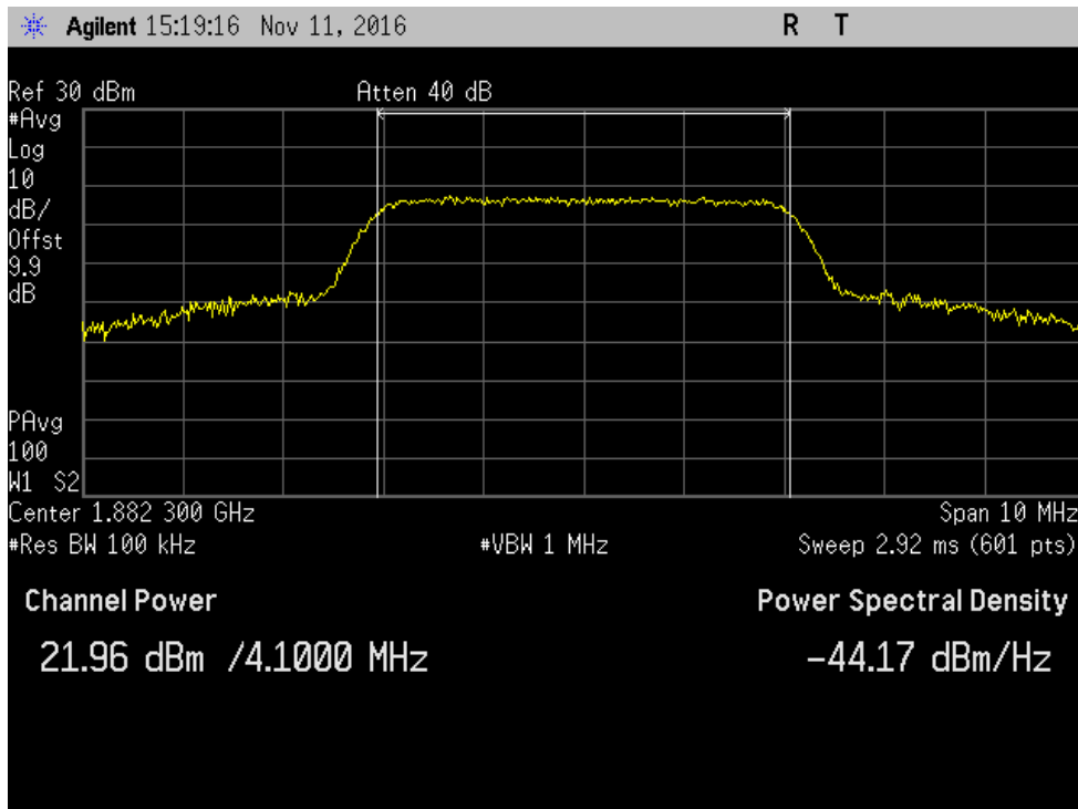
7.2_Power_UL_1850-1915MHz_AWGN_Max
