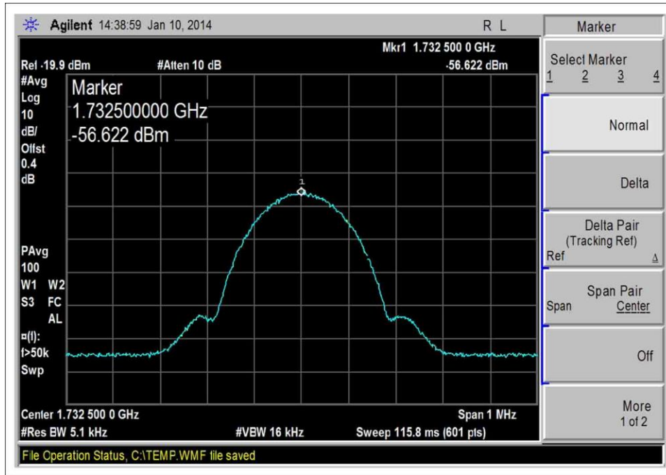
1710-1755 UL, GSM-Input
