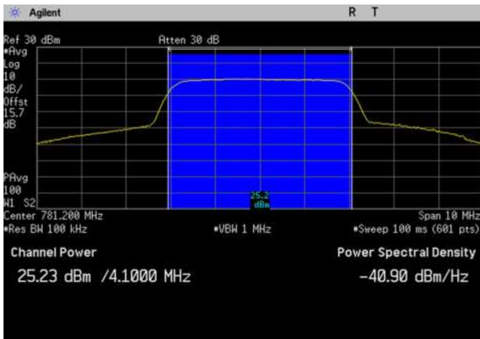
UL_776-787_AWGN_Max_781.2MHz
