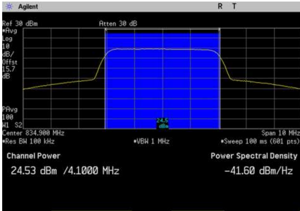
UL_824-849_AWGN_834.9MHz
