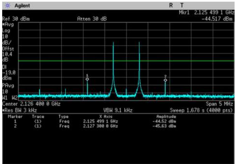
DL_2110-2155_2126.4MHz
