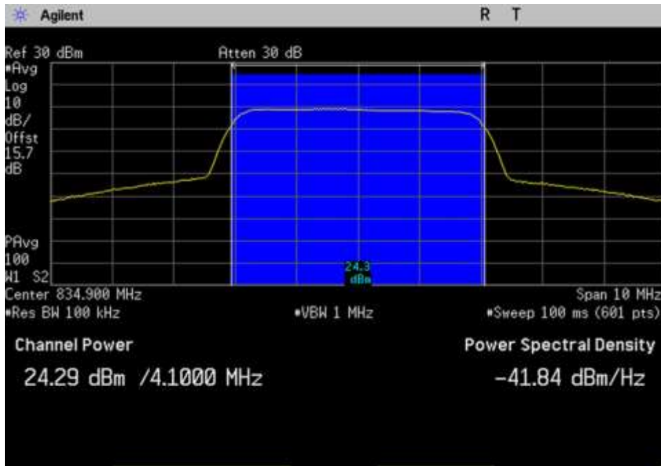
UL_824-849_AWGN_Max_834.9MHz
