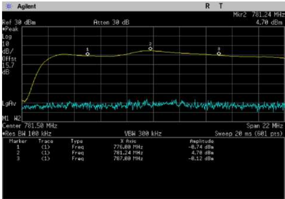
UL_776-787_ 776- 781.24MHz
