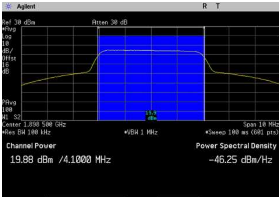
UL_1850-1915_AWGN_Max_1898.5MHz
