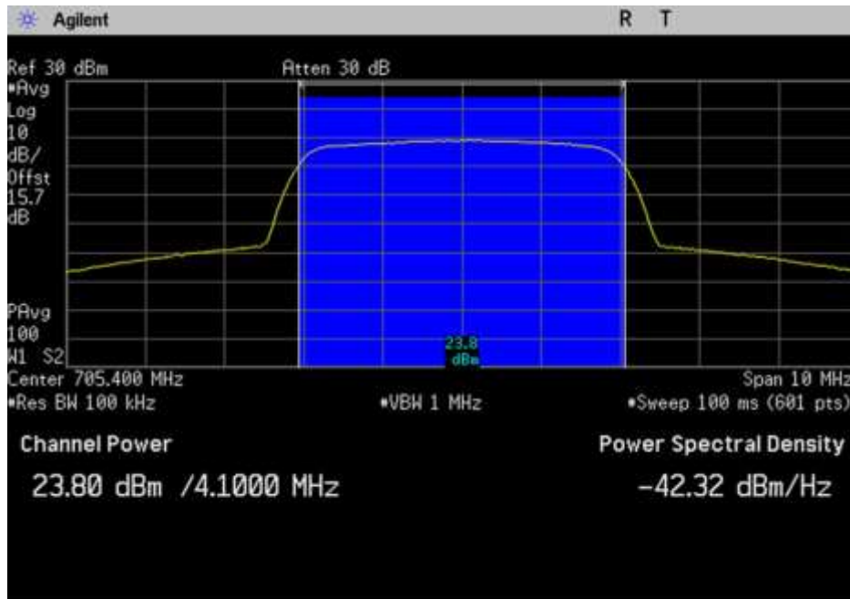
UL_698-716_AWGN_705.4MHz
