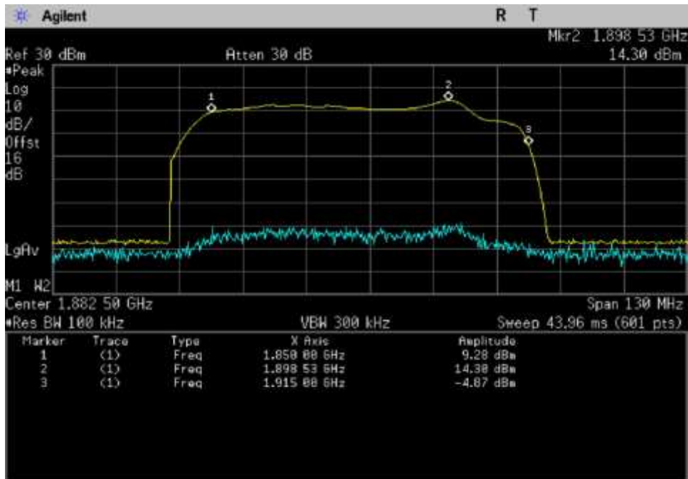
UL_1850-1915_1850-1898.53MHz
