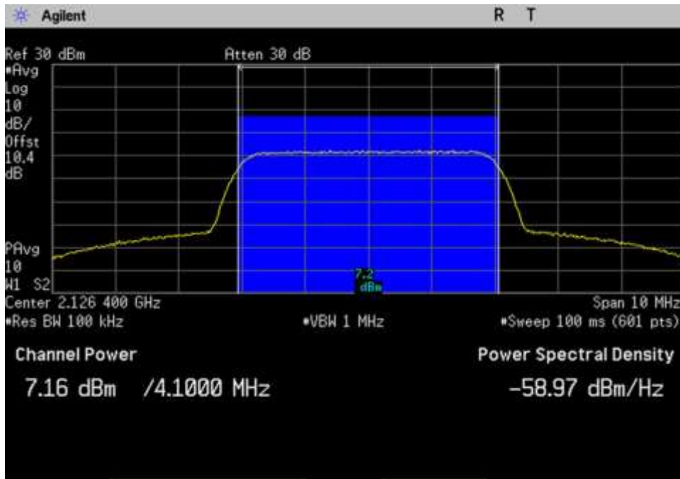
DL_2110-2155_AWGN_Max_2126.4MHz
