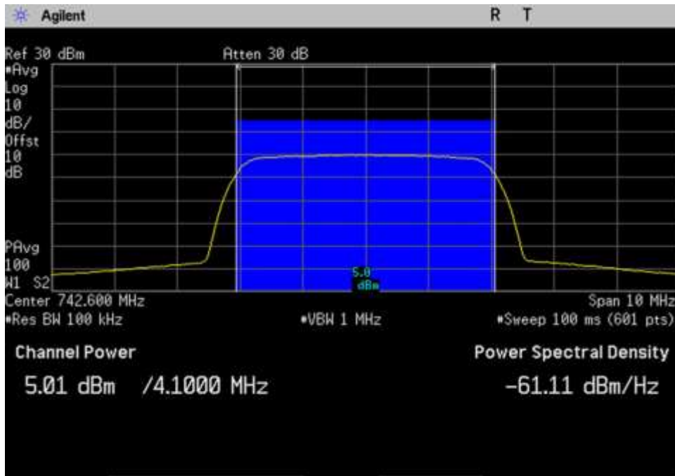
DL_728-746_AWGN_Max_742.6MHz
