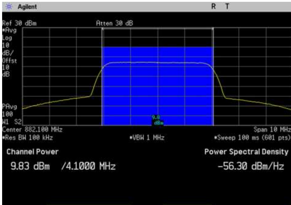
DL_869-894_AWGN_Max_882.1MHz
