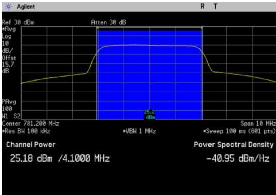
UL_776-787_AWGN_781.2MHz
