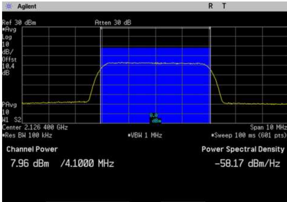
DL_2110-2155_AWGN_2126.4MHz
