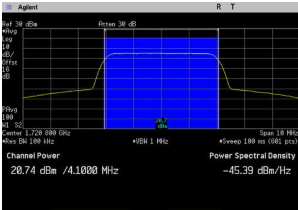
UL_1710-1755_AWGN_1720.8MHz
