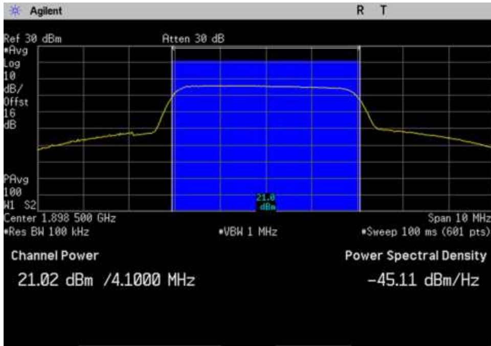
UL_1850-1915_AWGN_1898.5MHz
