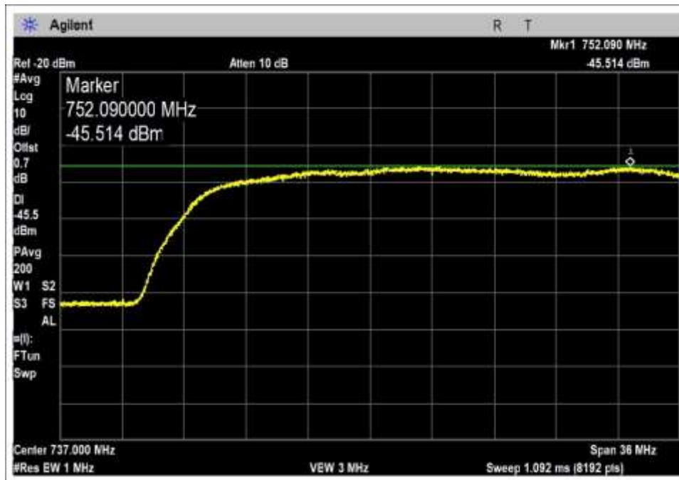
DL_728-746_ 737MHz
