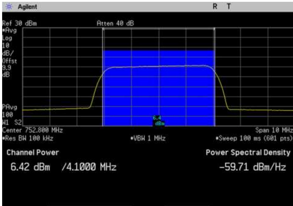
DL_746-757_AWGN_Max_752.8MHz
