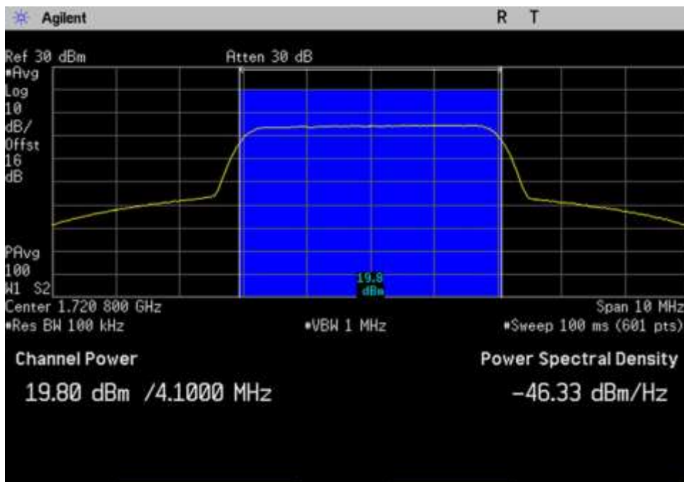
UL_1710-1755_AWGN_Max_1720.8MHz
