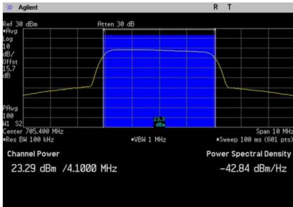
UL_698-716_AWGN_Max_705.4MHz
