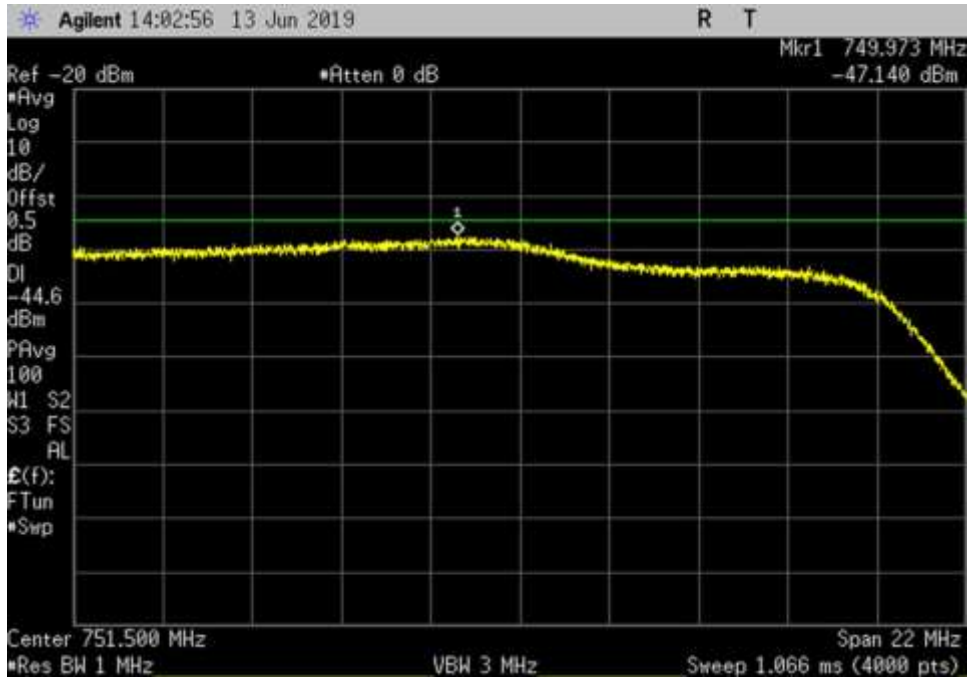
DL_746-757_751.5MHz_165ft Cable
