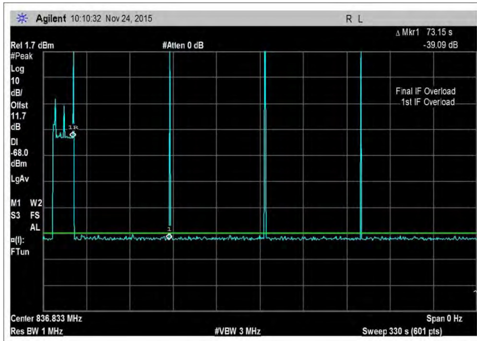
7.11_osc_UL-824-849MHz-330sec
