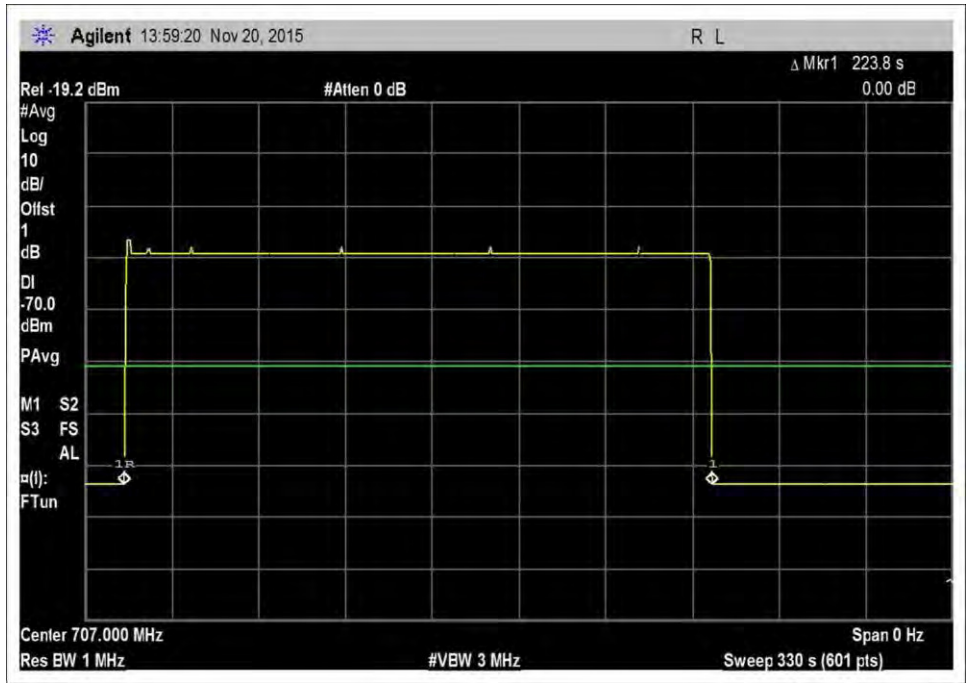
7.8_Inactivity_UL_698-707MHz
