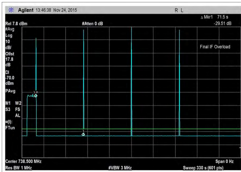
7.11_osc_DL-728-746MHz-330sec
