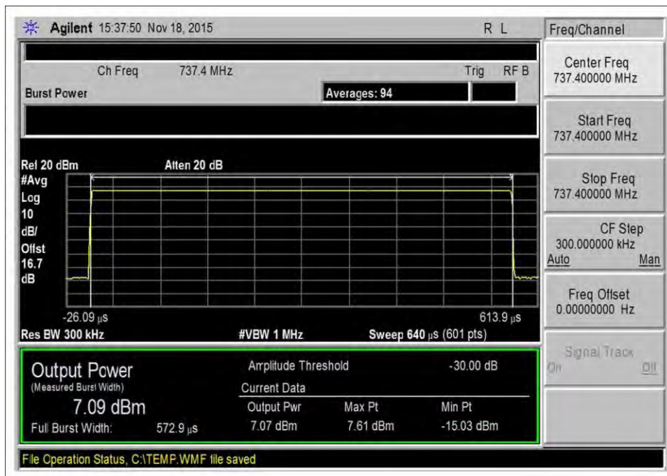
7.2_Power_DL_728-746_GSM-Max
