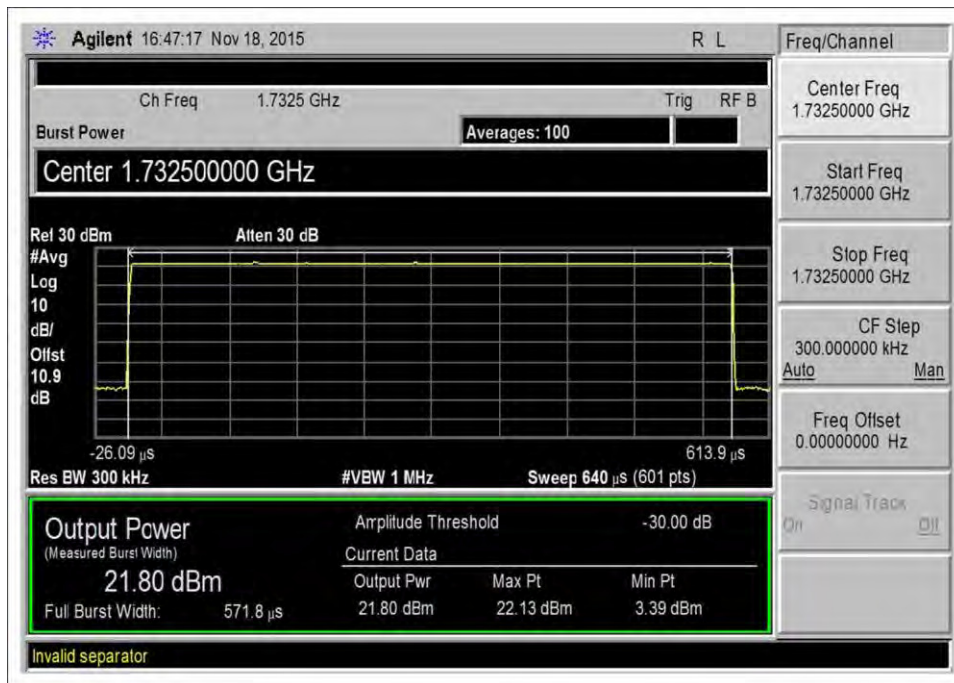
7.2_Power_UL_1710-1755_GSM
