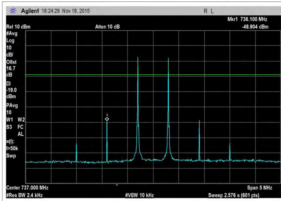
7.4_Intermod_DL_728-746MHz
