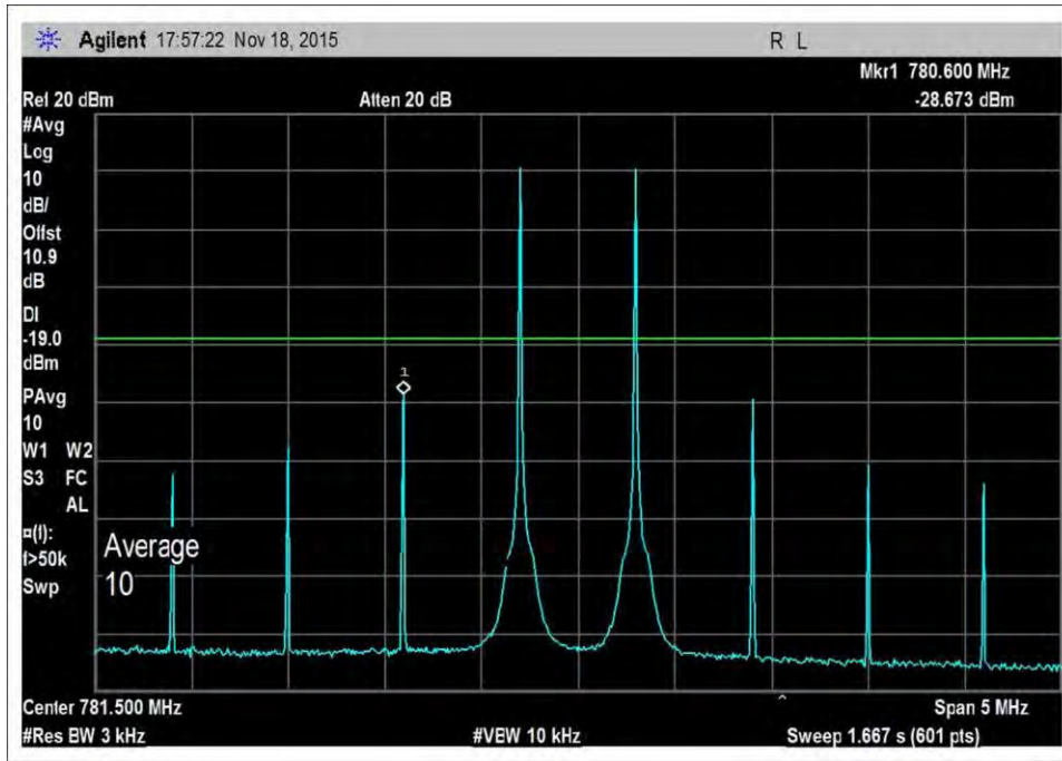
7.4_Intermod_UL_776-787MHz
