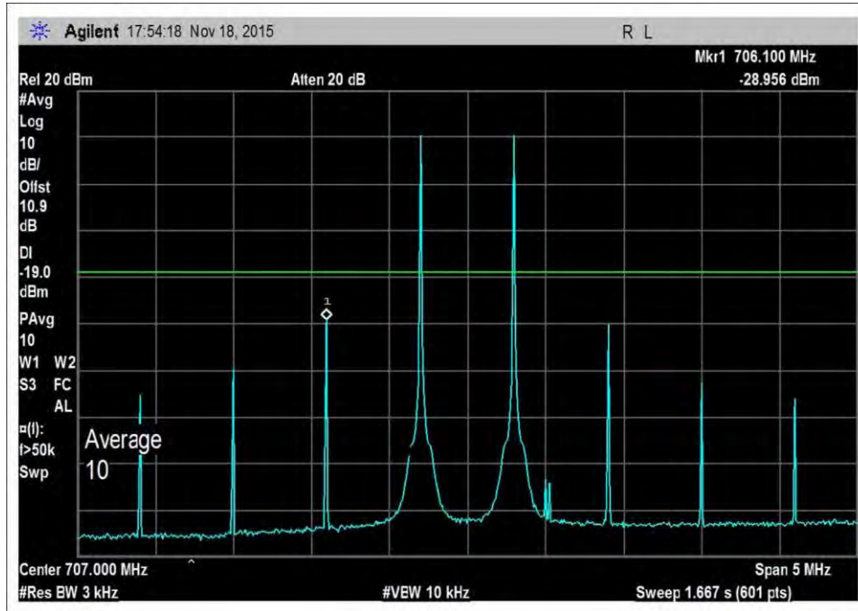
7.4_Intermod_UL_698-716MHz
