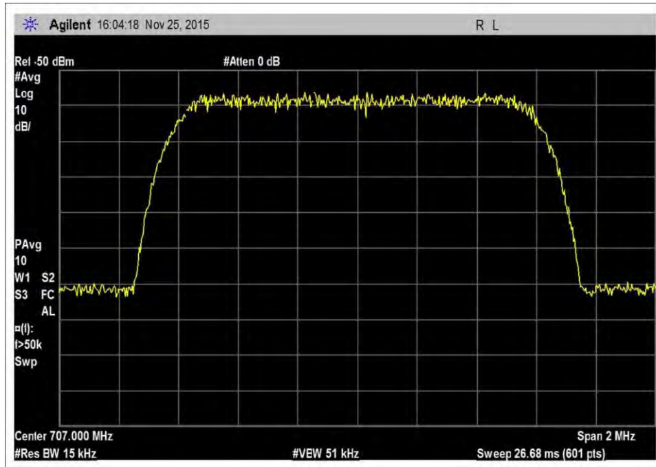
7.10_OBW_UL_698-716MHz_CDMA
