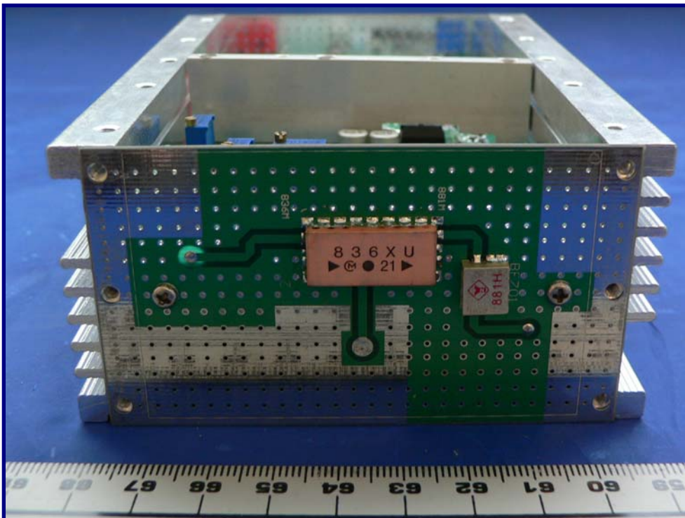
1.8 End View 2
