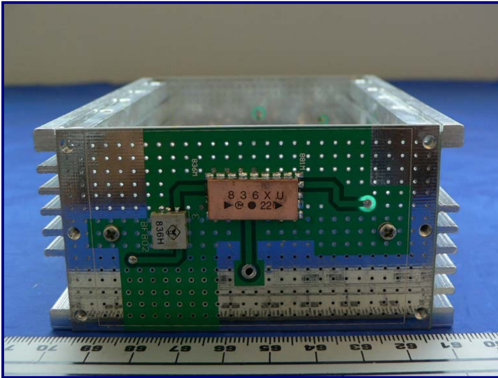
1.8 End View 2
