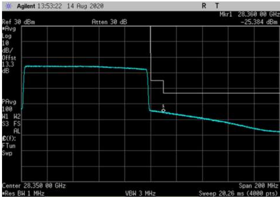
UL_27500-28350-64QAM-100MHz-H-CP OFDM_HC
