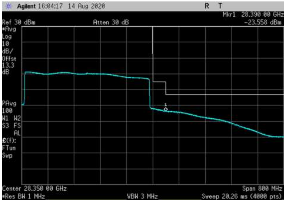
DL_27500-28350_QPSK-400MHz-H-CP OFDM_HC
