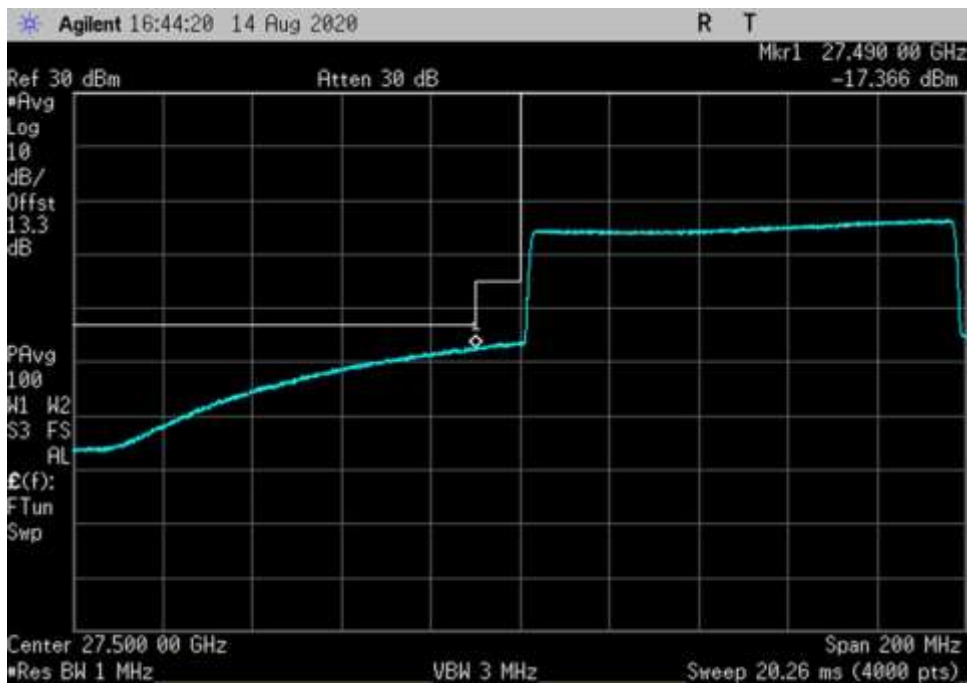
DL_27500-28350_64QAM-100MHz-H-AGC+3-CP OFDM_LC
