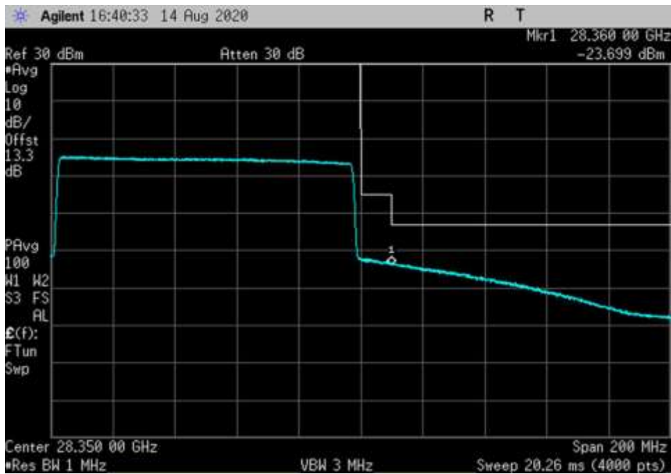
DL_27500-28350_64QAM-100MHz-H-AGC+3-CP OFDM_HC
