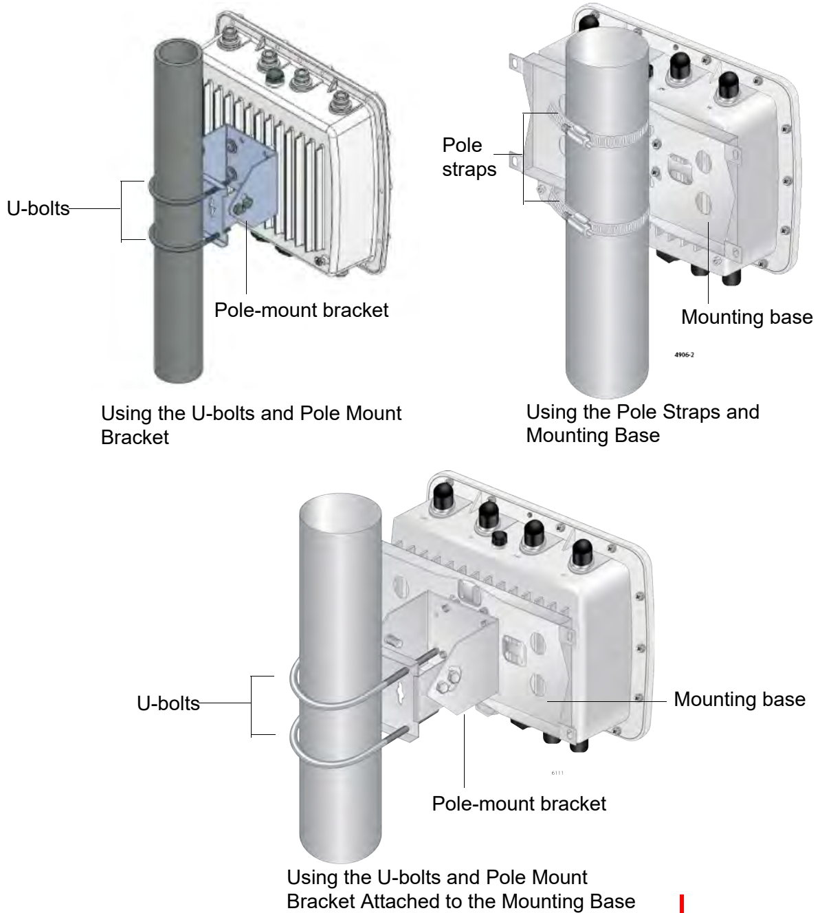
Figure 30. Three Methods of Pole Installations
