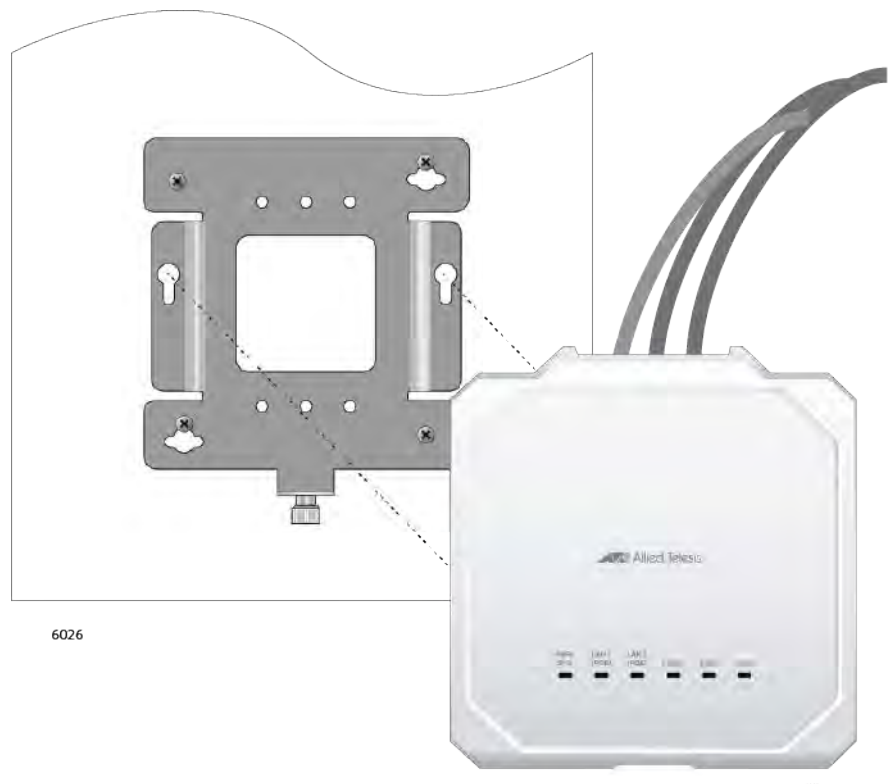
Figure 25. Installing the Access Point on the Mounting Bracket
