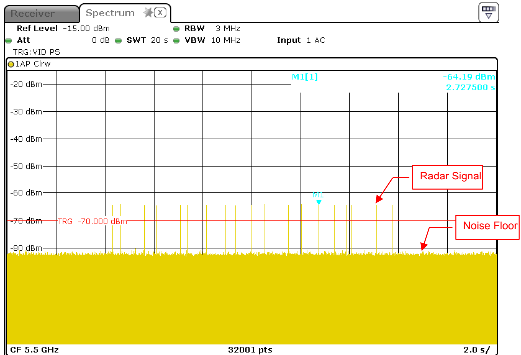
Radar Signal 5
