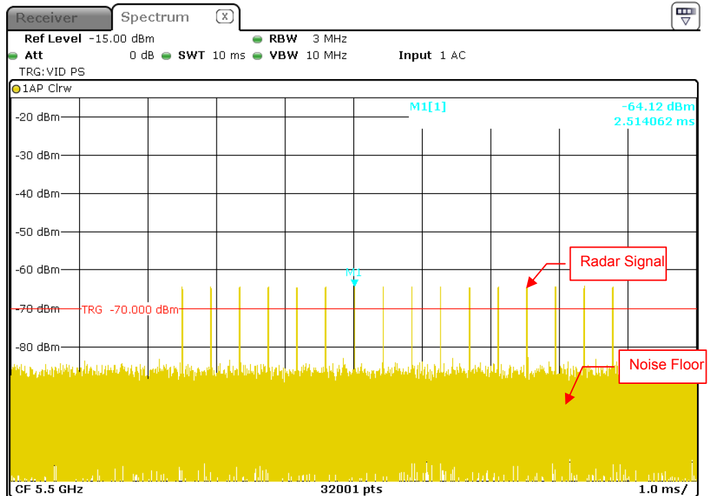
Radar Signal 3
