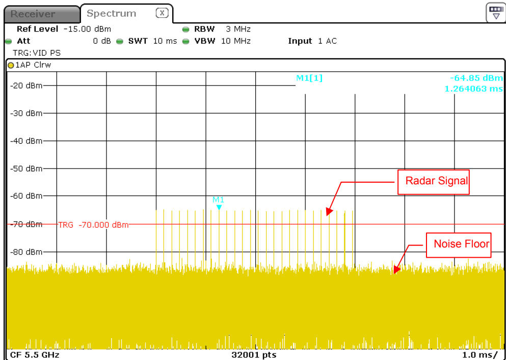
Radar Signal 2
