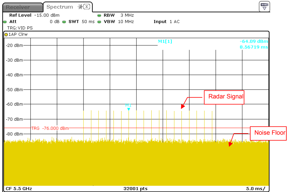
Radar Signal 0
