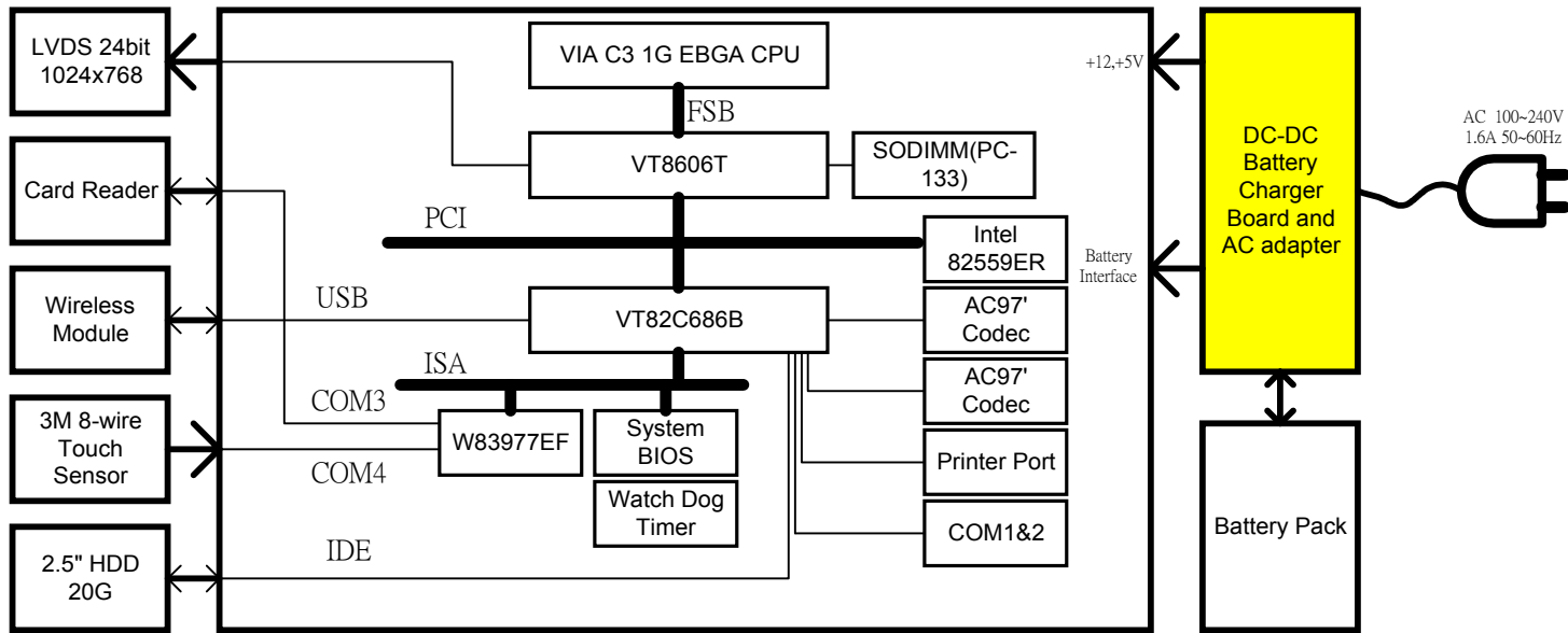
Figure1: ATP-151 Model block diagram
