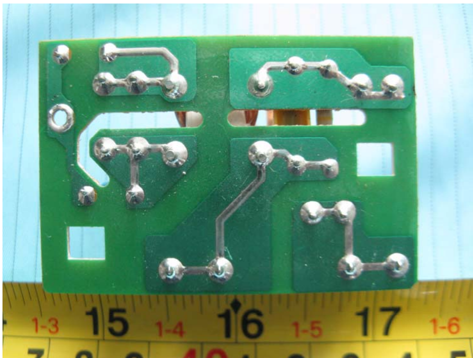
EUT – EMI Filter Board Bottom Circuit View
