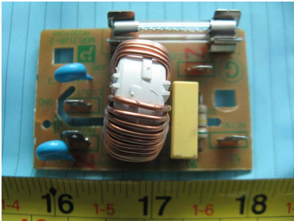
EUT – EMI Filter Board Top Components View
