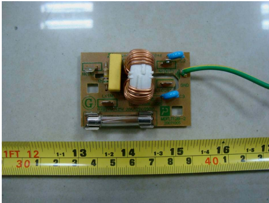
EUT – EMI Filter Board Circuit View
