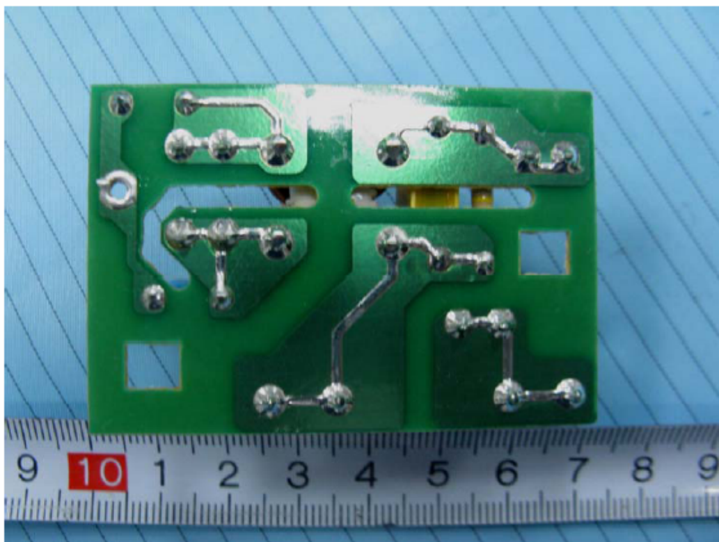
EUT – EMI Filter Board Bottom Circuit View
