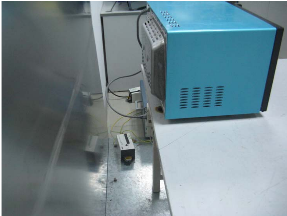
Conduction Emissions - Rear View
