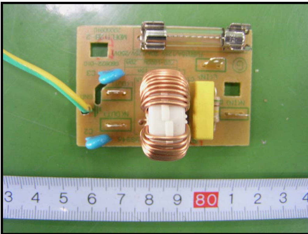
EUT – Power board Components View
