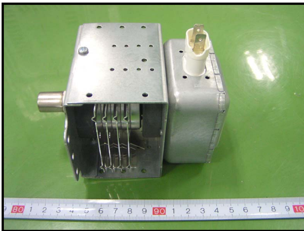
EUT -Emitter Side View
