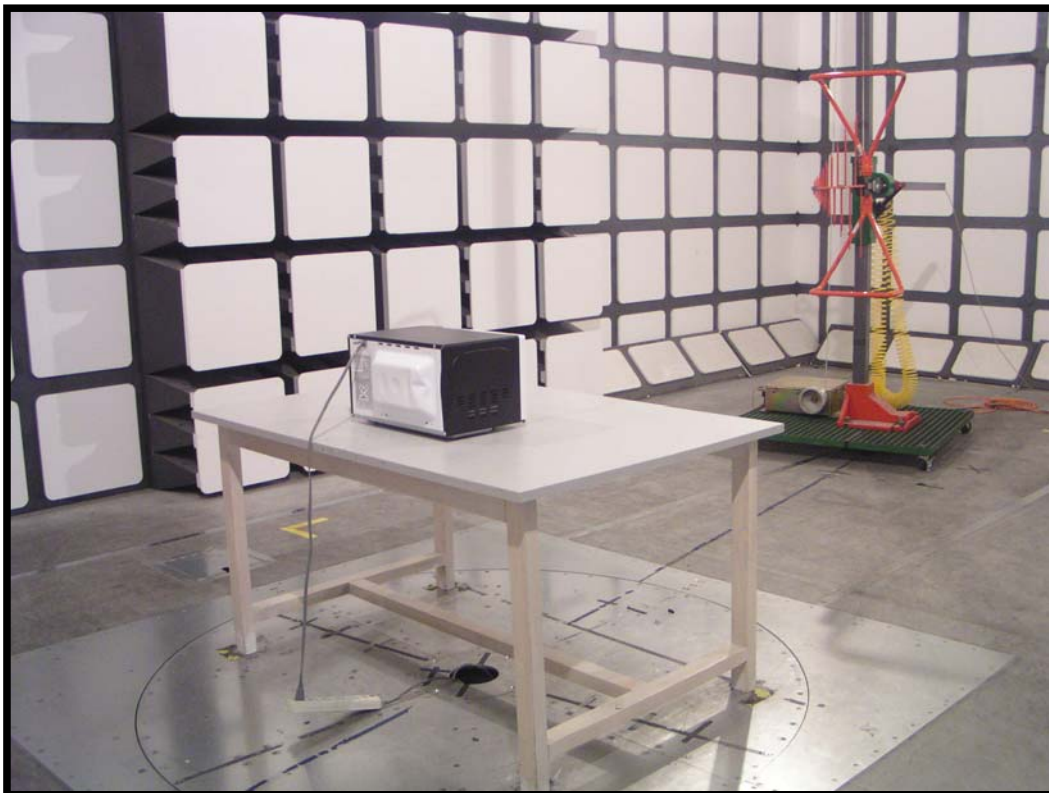
Radiated Emissions - Rear View (30 to 1000MHz)
