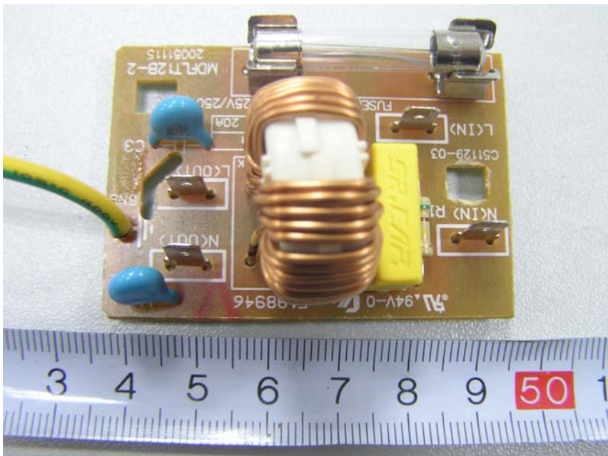
EUT – Power Input PCB Front View
