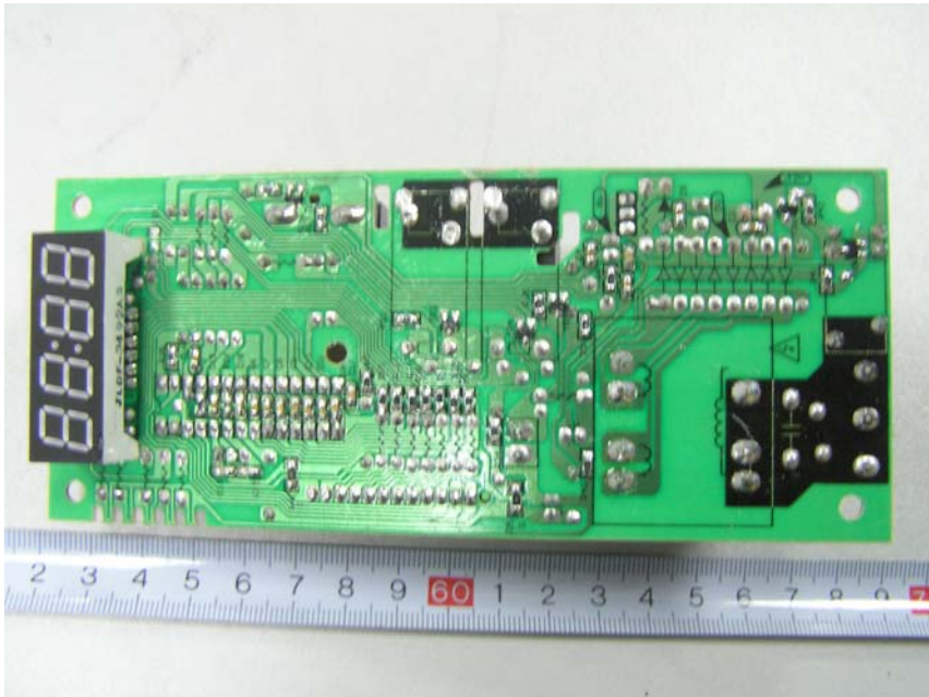
EUT – Main Board PCB Back View
