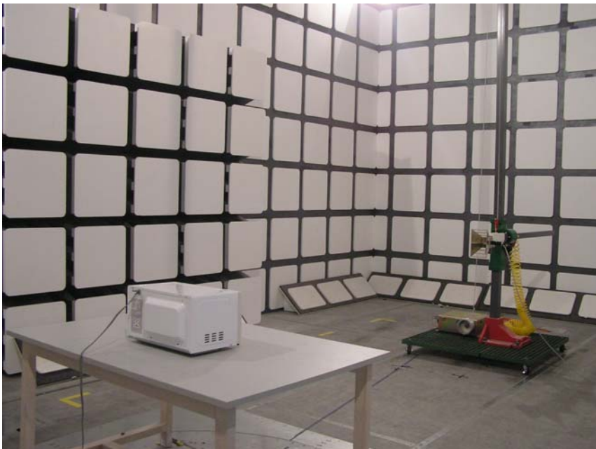
Radiated Emission (Above 1 GHz) - Rear View
