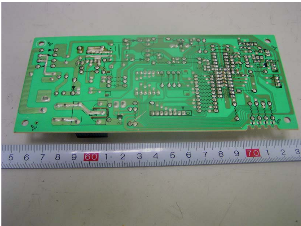
EUT – Control Board Bottom Components View
