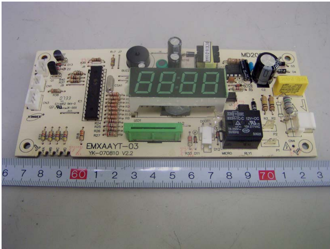
EUT – Control Board Top Components View
