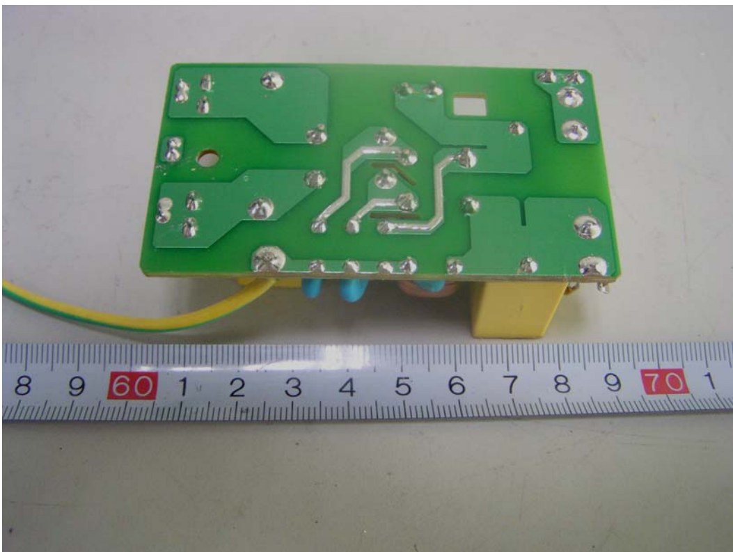
EUT – Filter Board Circuit View
