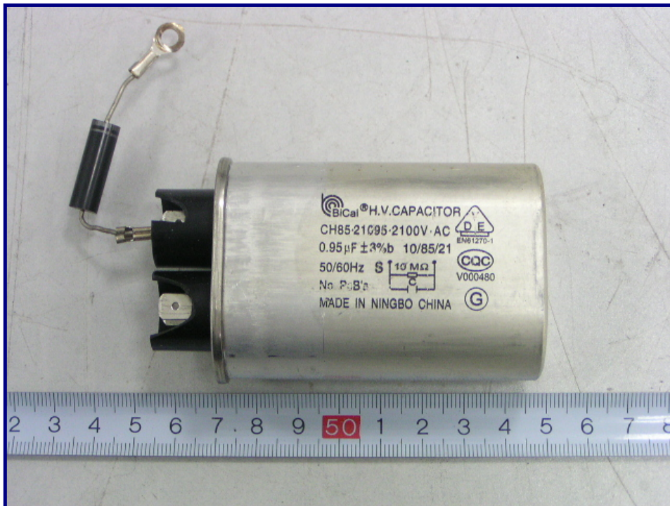
EUT –Filter View
