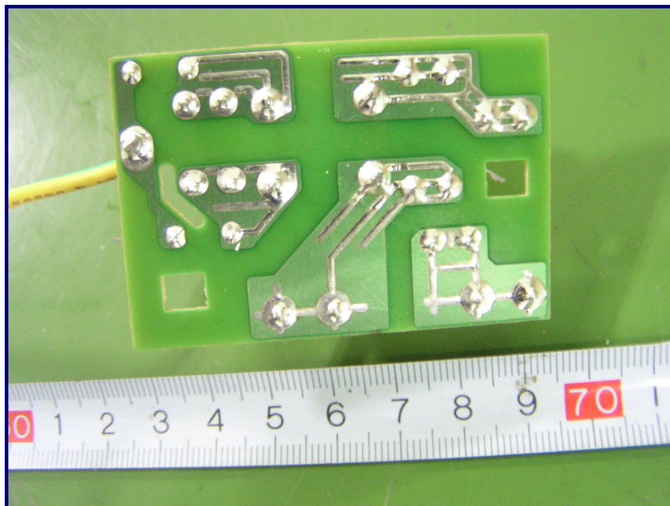
EUT –Filter Board Circuit View
