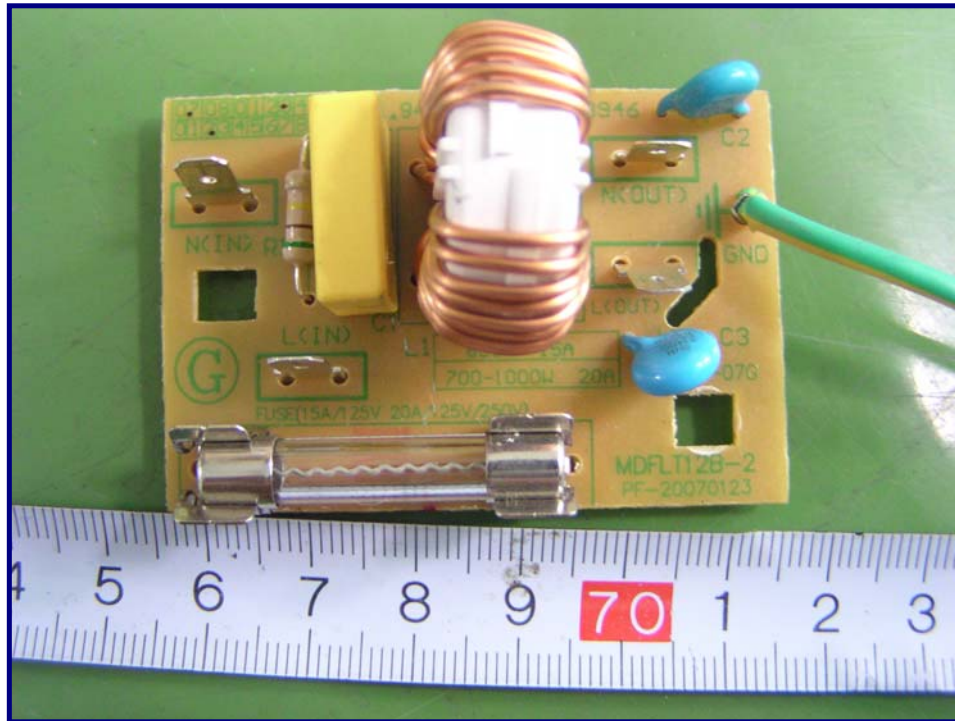
EUT –Filter Board Components View
