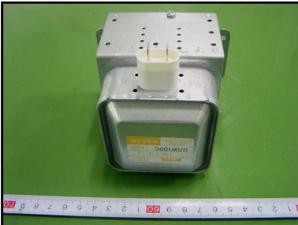
EUT –Emitter Front View
