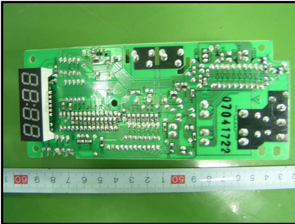
EUT - Control Panel board Circuit View
