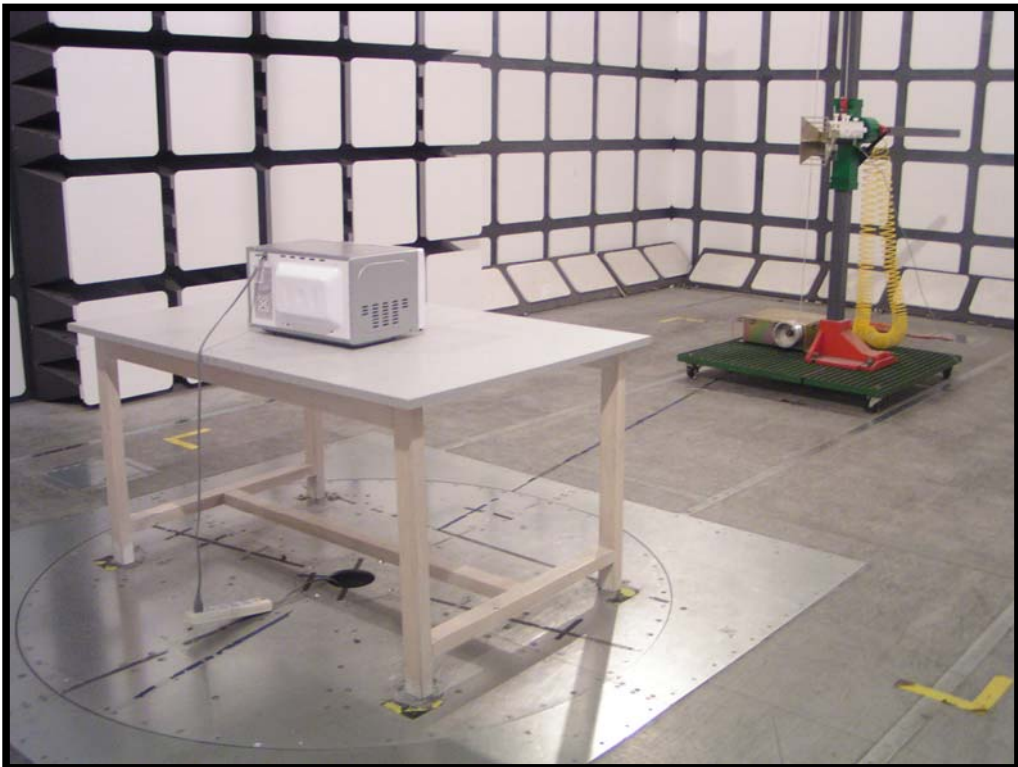
Above 1 GHz: Radiated Emissions - Rear View
