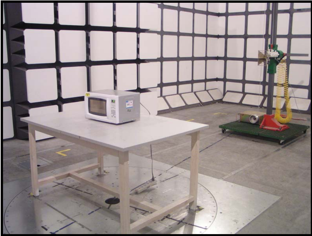
Above 1 GHz: Radiated Emissions - Front View
