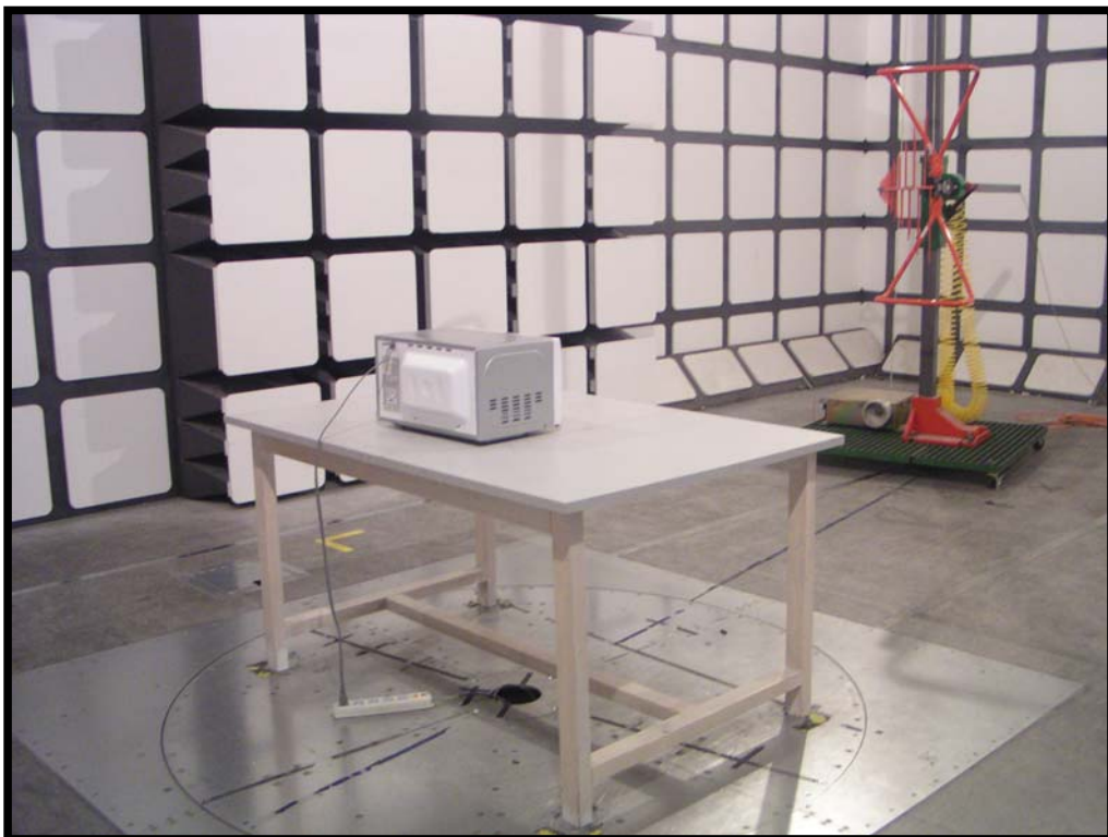
30MHz to 1000MHz: Radiated Emissions - Rear View
