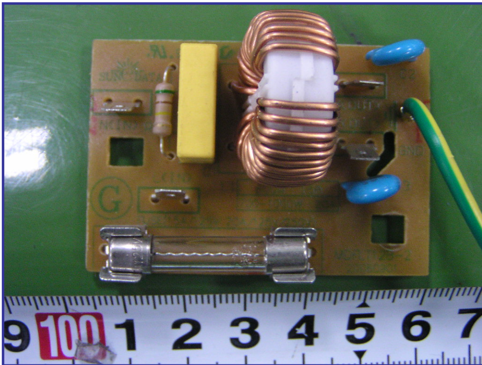
EUT – EMI PCB Component View
