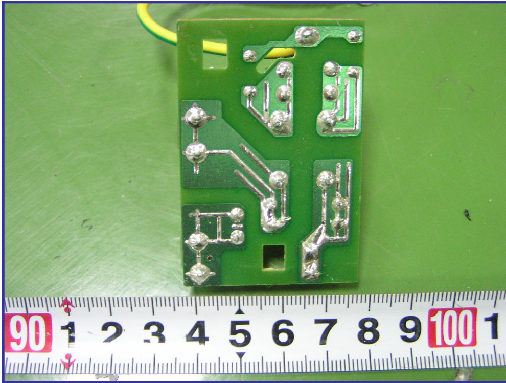
EUT – EMI PCB Circuit View
