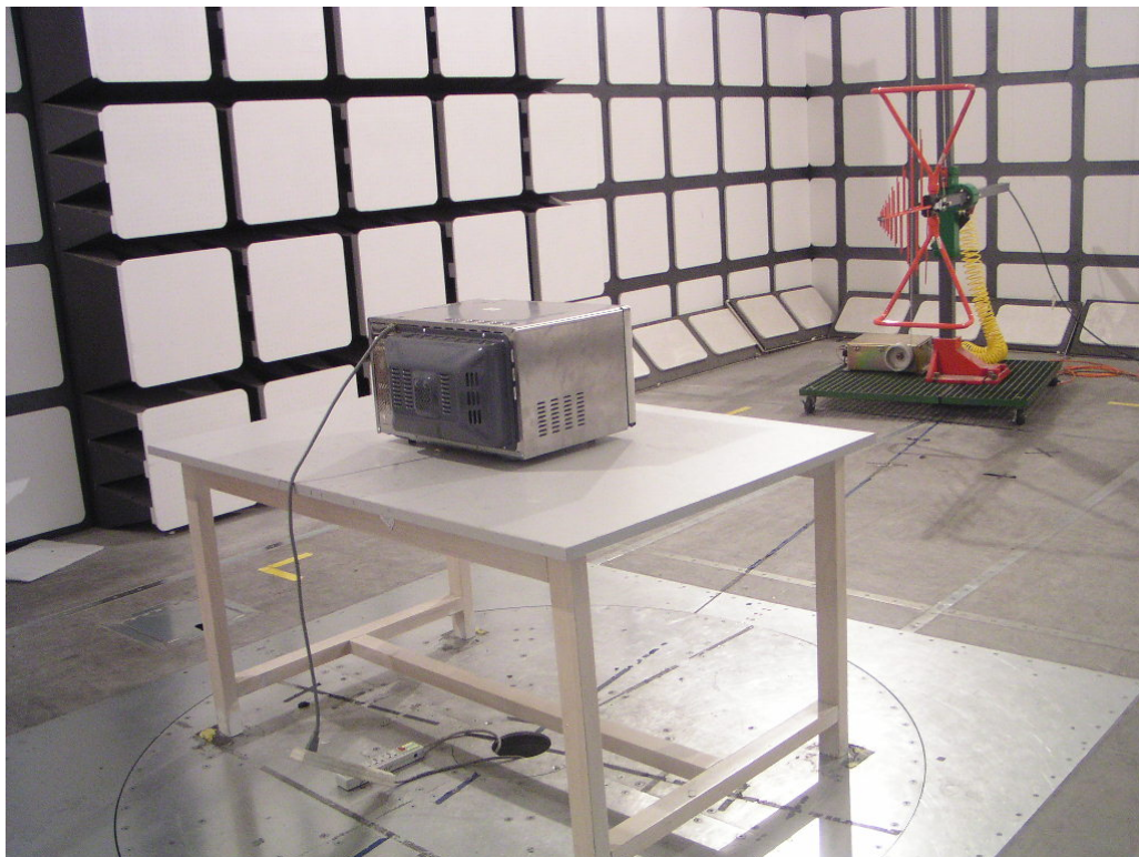
30MHz-1000MHz: Radiated Emissions - Rear View
