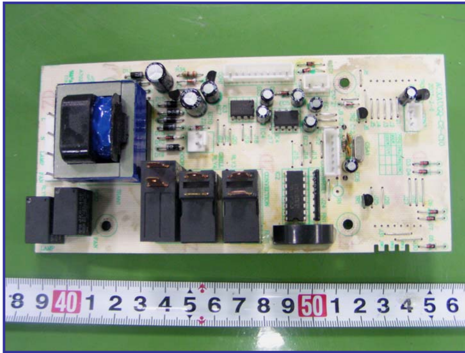
EUT – Power PCB Top Component View
