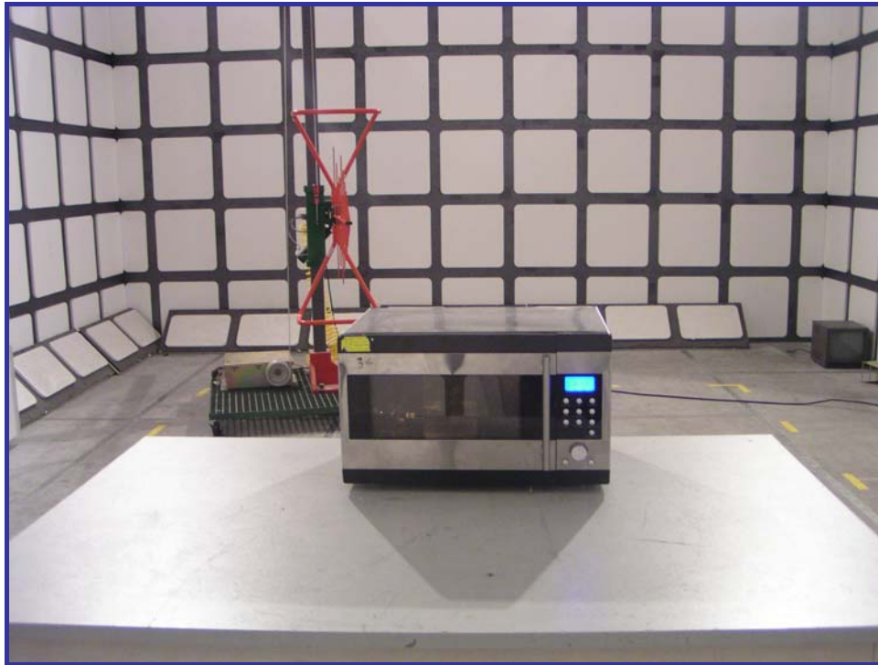
30MHz to 1000MHz: Radiated Emissions - Rear View
