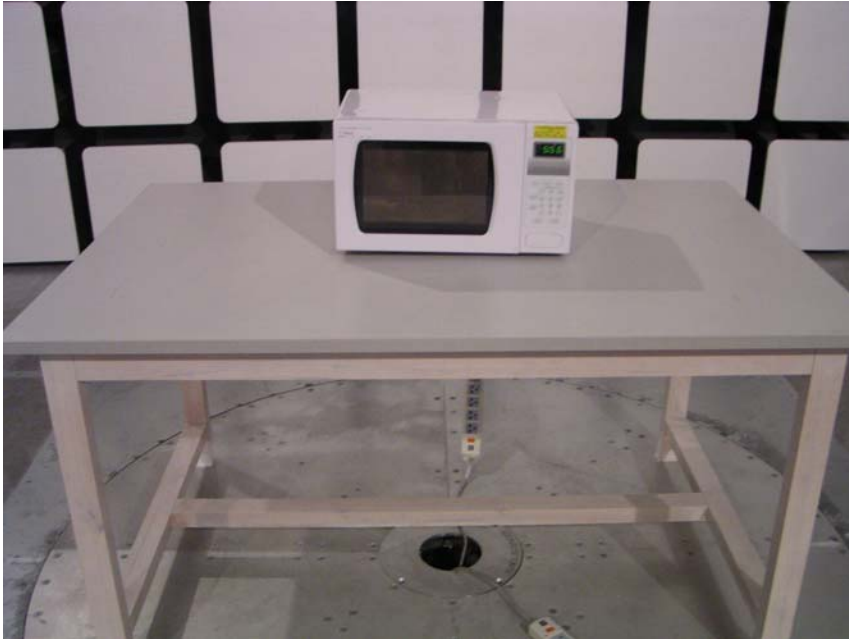
Radiated Emission–Front View (30MHz-1000MHz)
