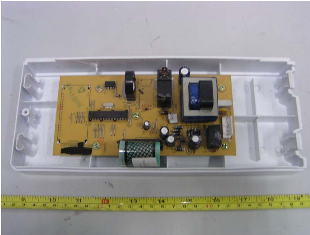
Internal photo-Uncover View-3
