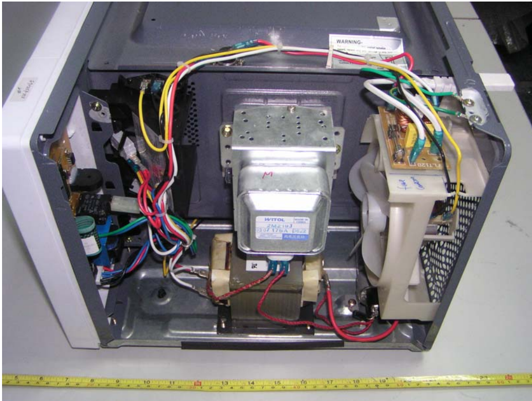
Internal photo-Uncover View-1
