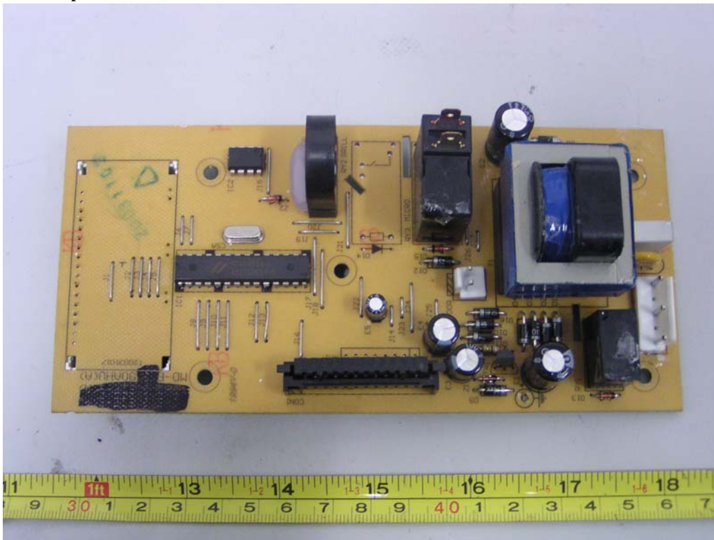
Internal photo-PCB View-1
