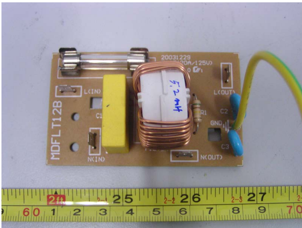
Internal photo-PCB View-3
