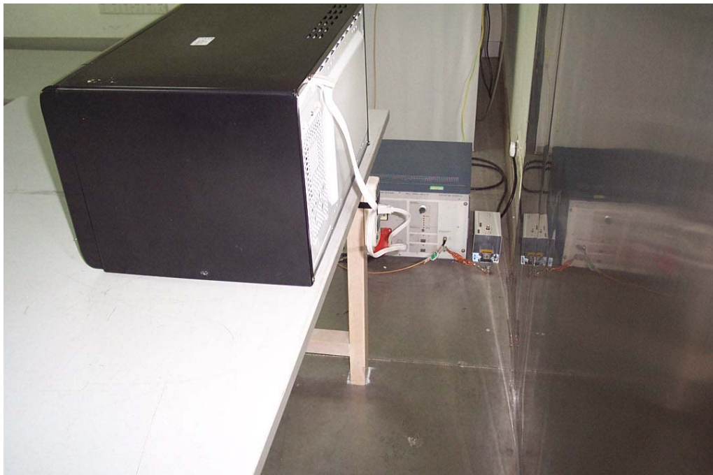
Conducted Emission - Rear View
