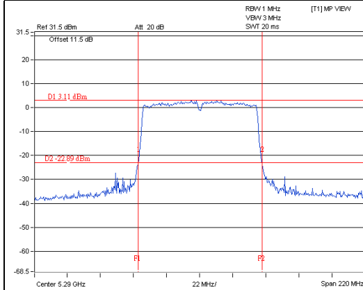
11ac (80MHz) 1S3T TxBF CH58 Chain2
