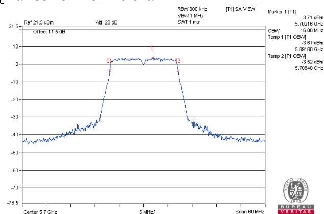
11a 1S3T CDD CH140 Chain3
