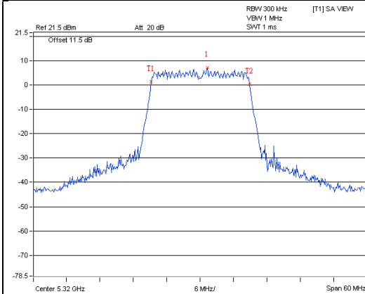
11ac (20MHz) 3S3T SDM CH64 Chain3
