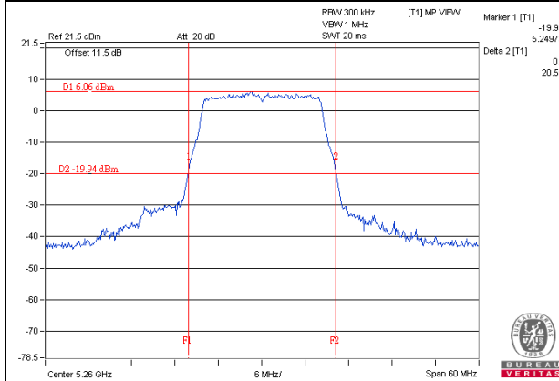
11a 1S3T CDD CH52 Chain2
