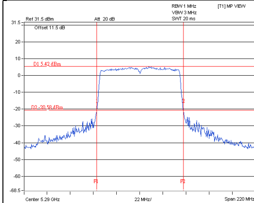
11ac (80MHz) 1S3T TxBF CH58 Chain3
