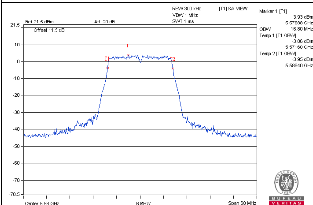
11a 1S3T CDD CH116 Chain3
