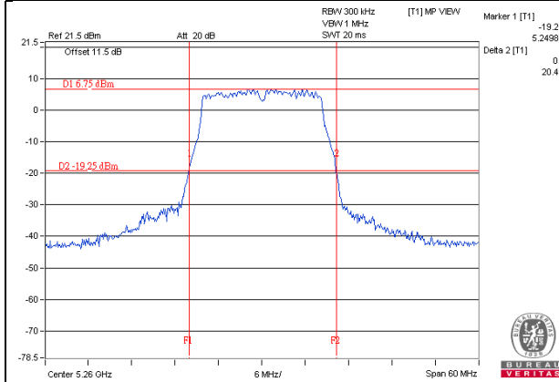
11a 1S3T CDD CH52 Chain3
