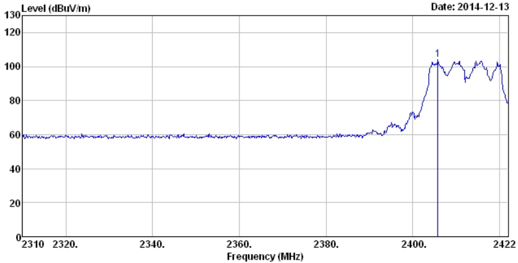
Plot on Configuration IEEE 802.11g / 6Mbps / CH1 / Ant.1+2 CDD mode / Reference Level
