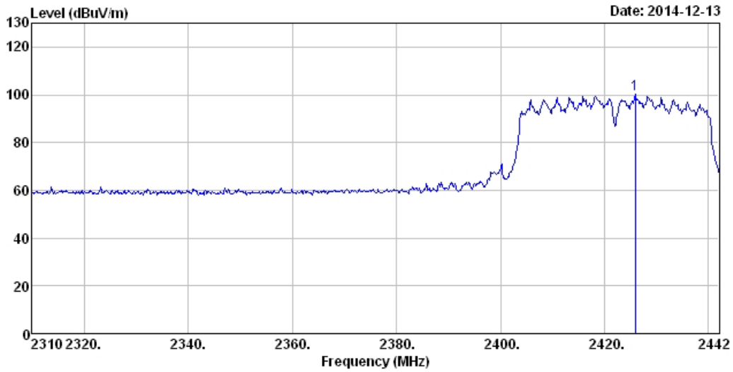
Plot on Configuration IEEE 802.11n 40MHz MCS0 / CH3 / Ant.1+2 CDD mode / Reference Level
