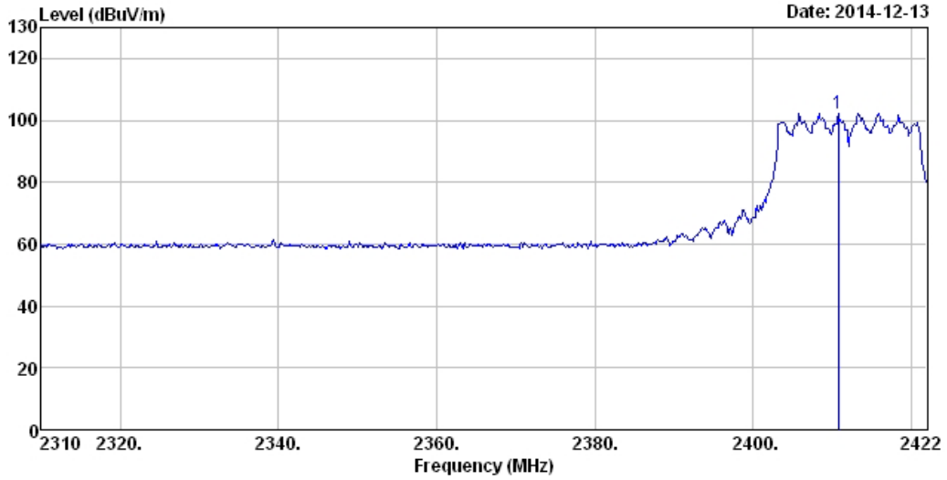
Plot on Configuration IEEE 802.11n 20MHz MCS0 / CH1 / Ant.1+2 CDD mode / Reference Level
