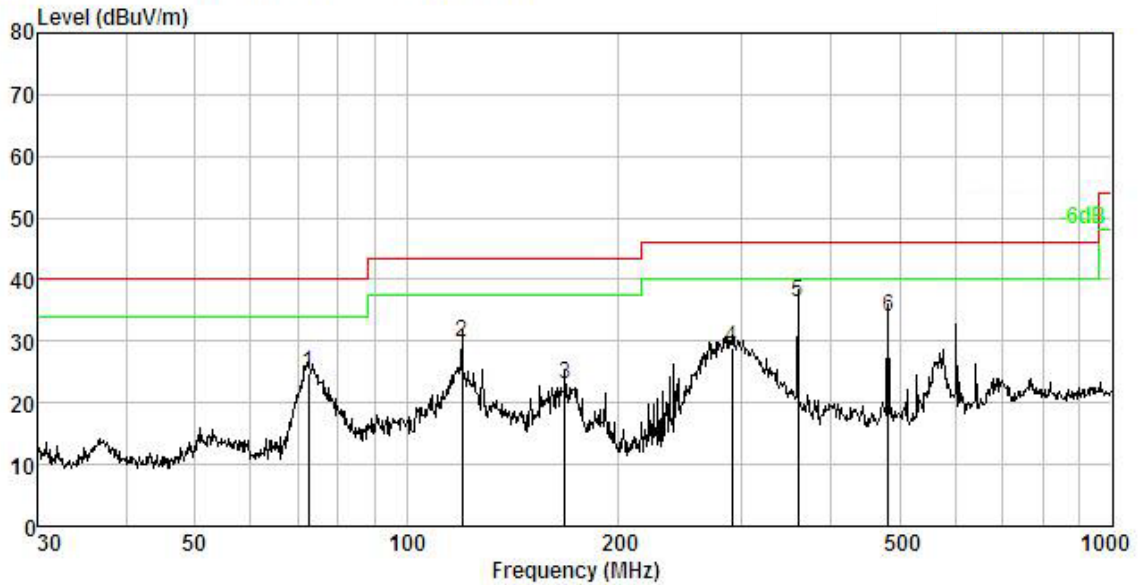
Test plot for Horizontal: Mode: GFSK (2441MHz)
