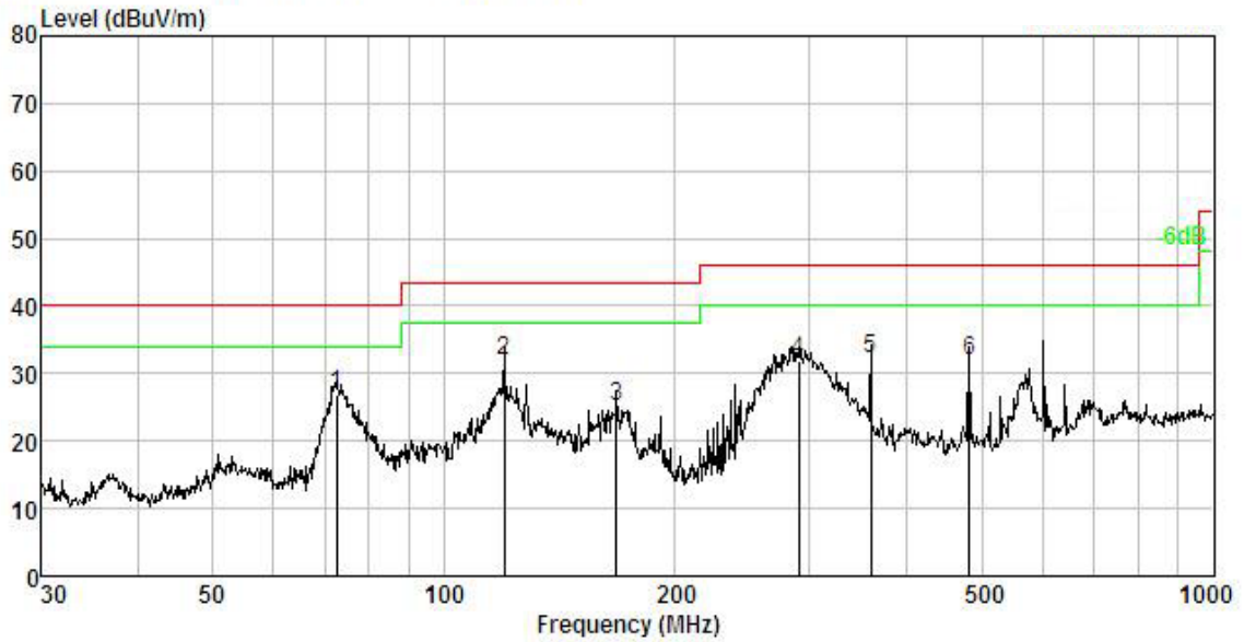
Test plot for Horizontal: Mode: GFSK (2480MHz)
