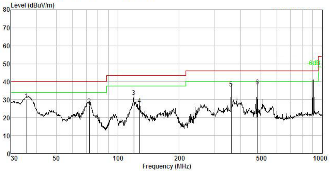
Test plot for Vertical: Mode: GFSK (2441MHz)
