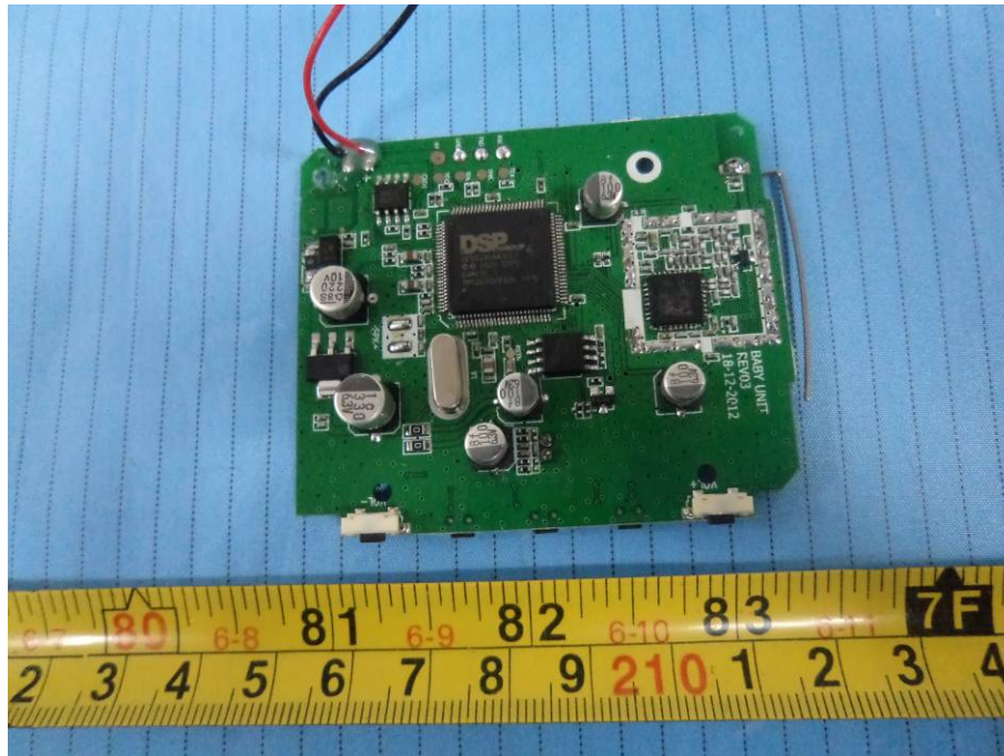
EUT (Baby Unit) – Main Board Top Shielding off View
