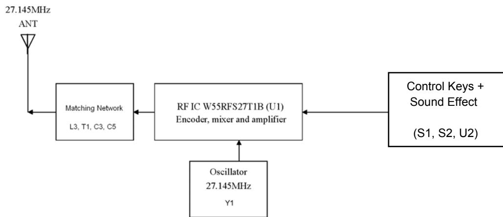
Transmitter Block Diagram Model no.: A1649
