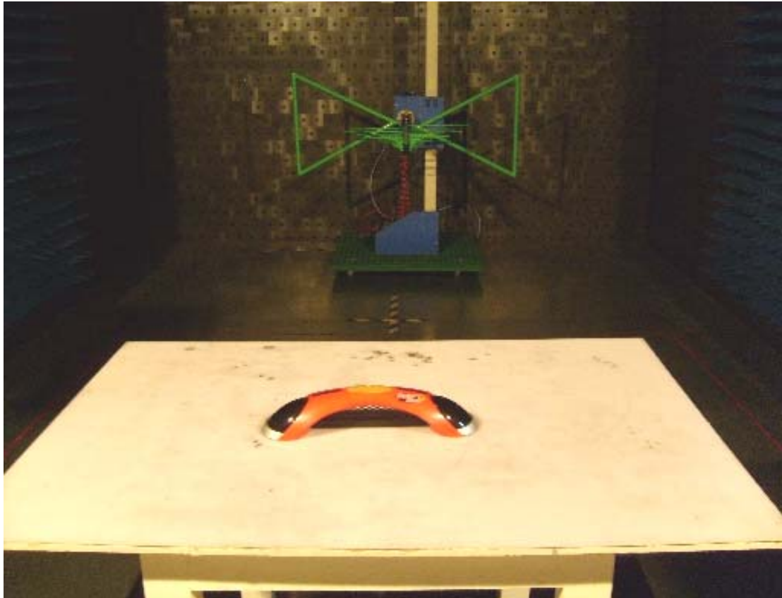
Radiated Emission above 30MHz
