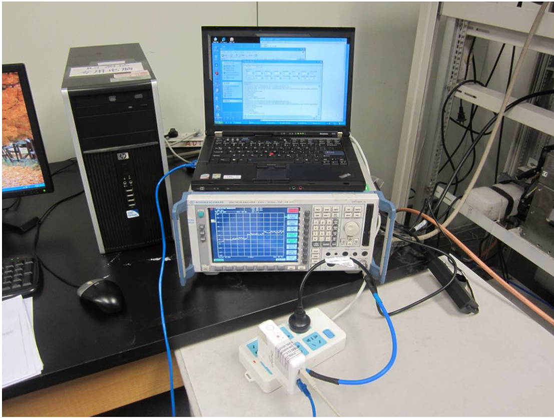
RF Setup photo
