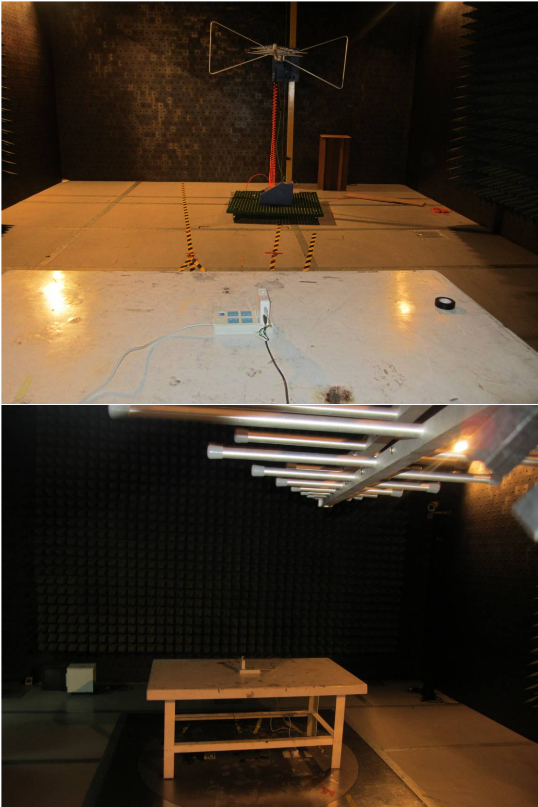
RE Setup photo
