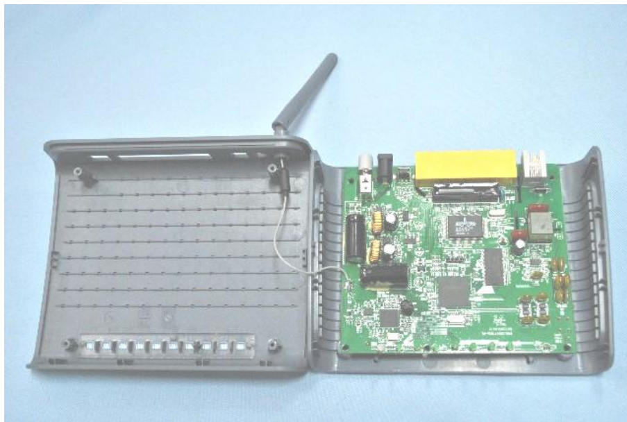
Main board component side
