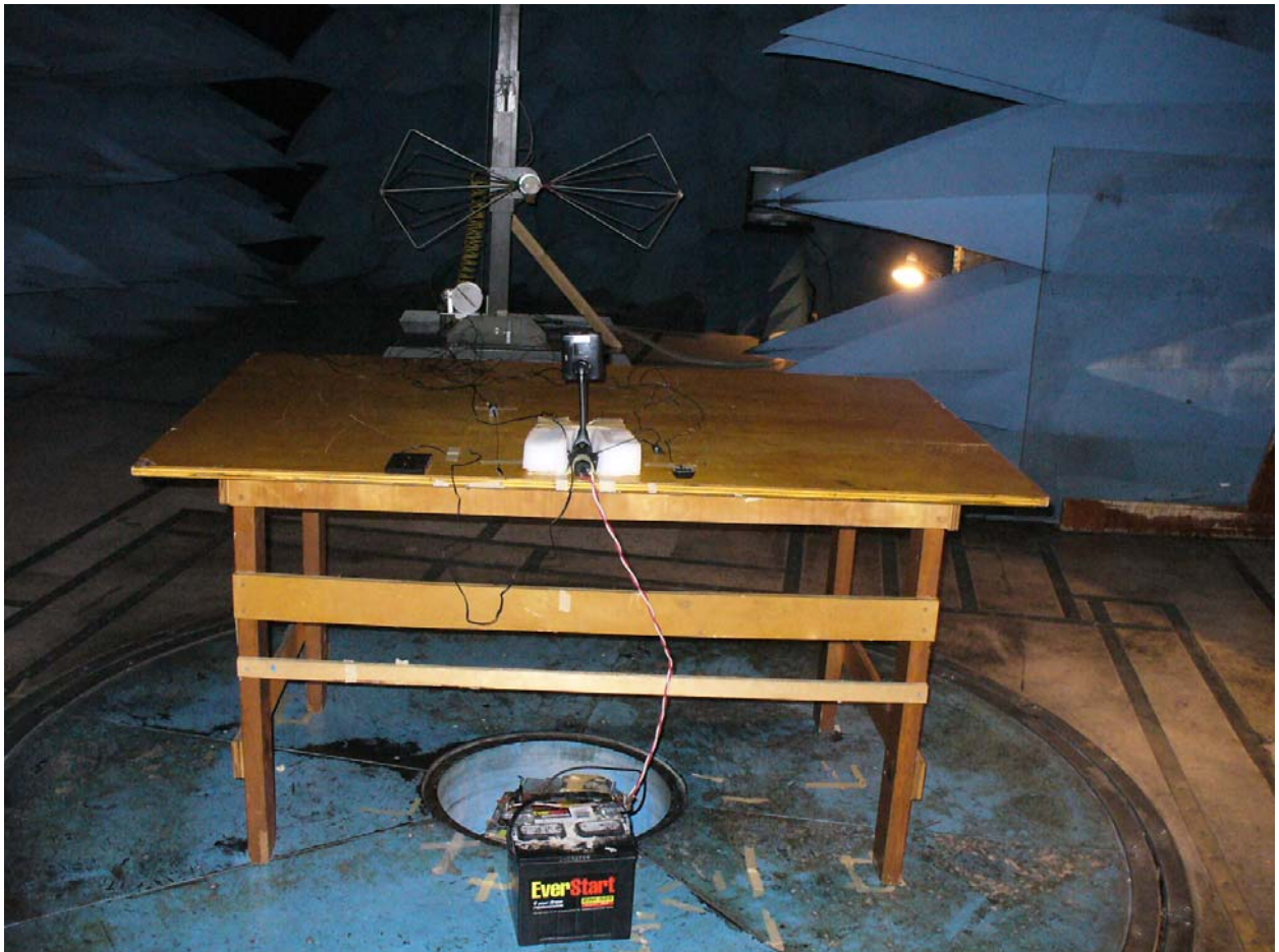
Figure 4: Back View
